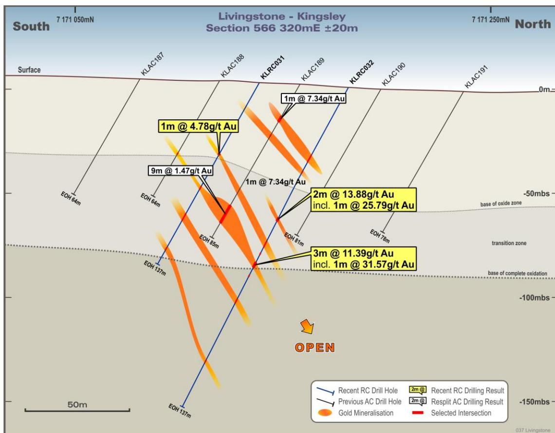
Figure 2: Section 566320mE
