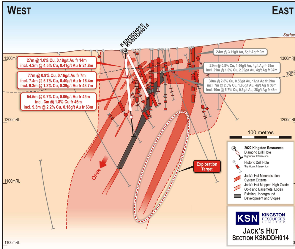
Figure: Jack's Hut Copper and gold target Cross Section KSNDDH014 and KSNDDH015
