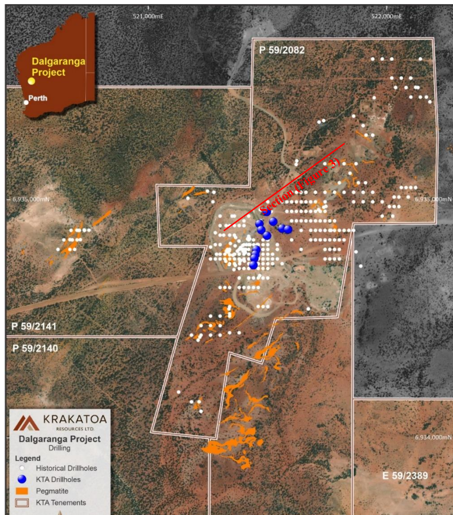
Figure 1 Dalgaranga Project historical mine zone showing areas of mapped pegmatites and extent of the drillholes within the area (historical and Krakatoa's). Section trace shown in red.
