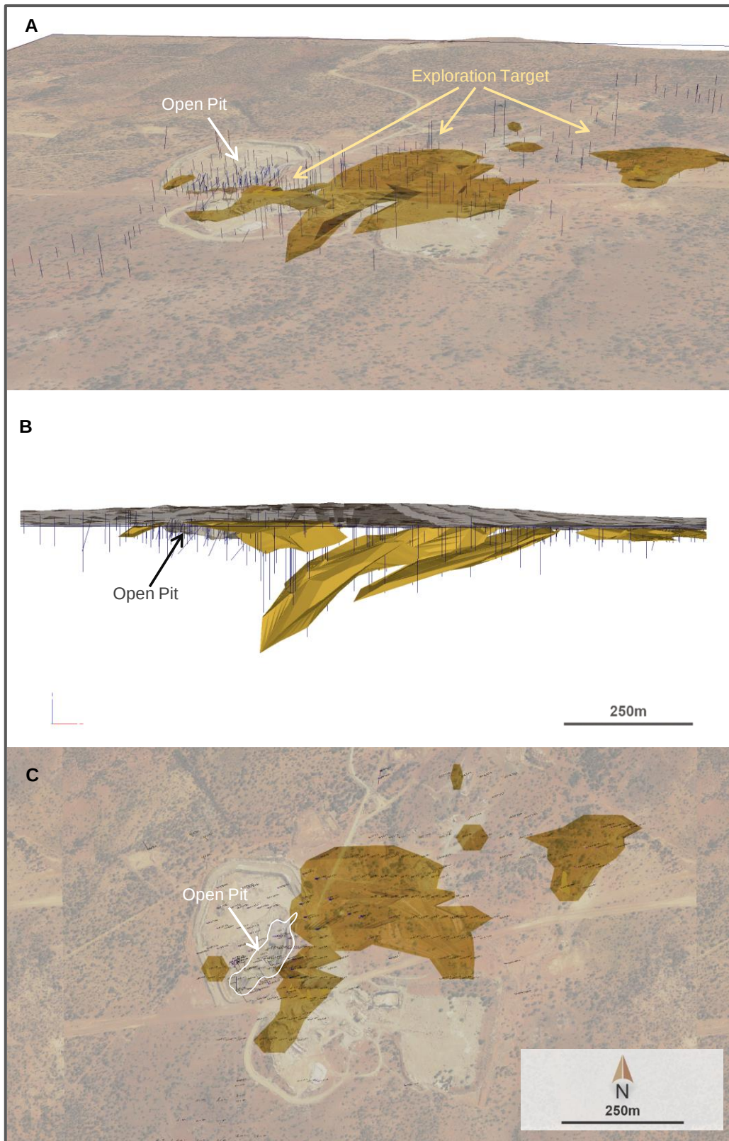
Figure 2 Geological model of pegmatite shown with transparent satellite image. A) Oblique view looking NNE indicating historical Open pit area and modelled Exploration Target. B) Cross section looking North showing drill trace, Exploration Target and area of open pit. C) Plan view showing aerial extent of Exploration Target and historical mine infrastructure.
