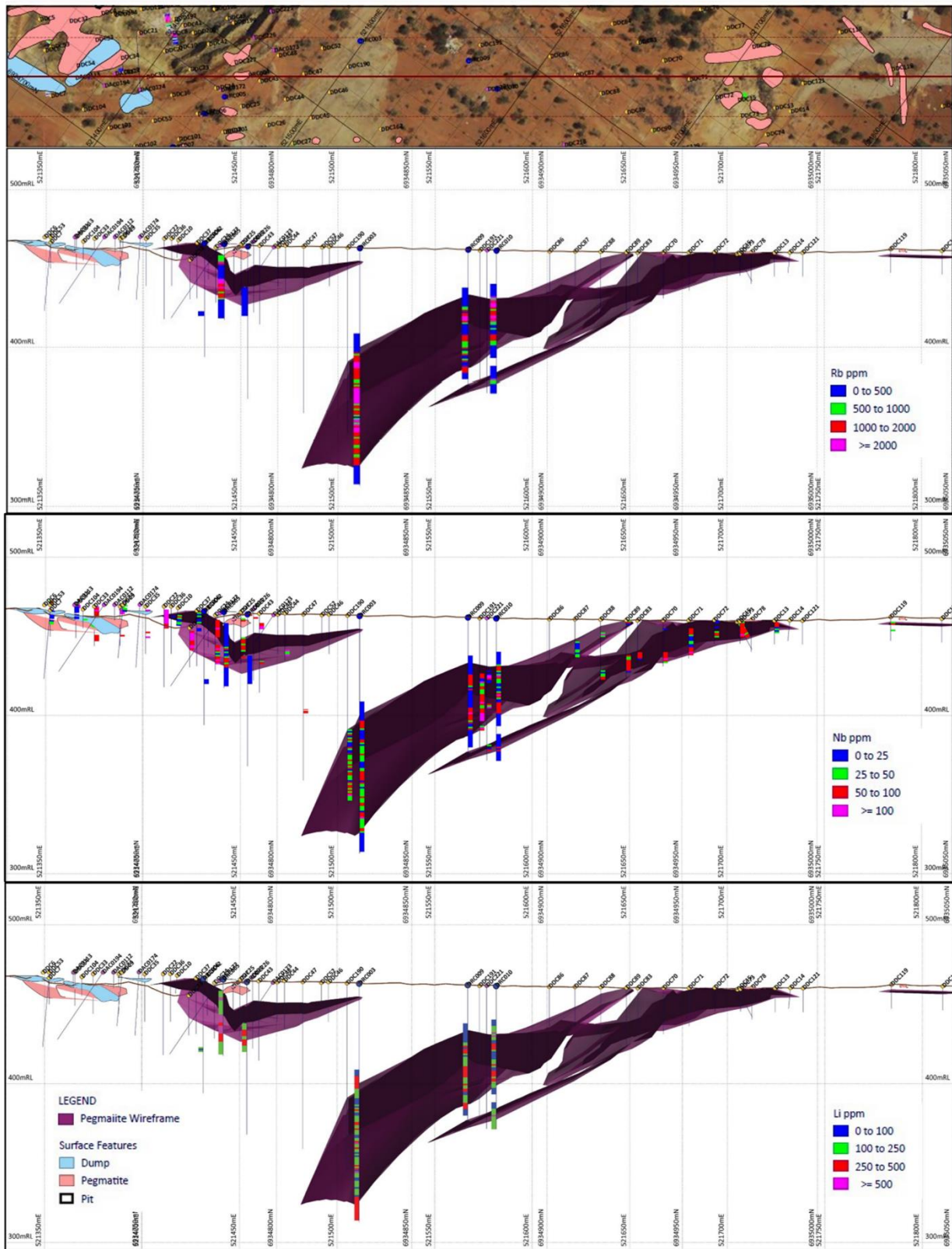
Figure 3 Dalgaranga downhole sections showing distribution of Rb (top) , Nb (middle) and Li (bottom) within the modelled pegmatite wireframe. Looking northwest, 25m to and away. Scale 1:1500.
