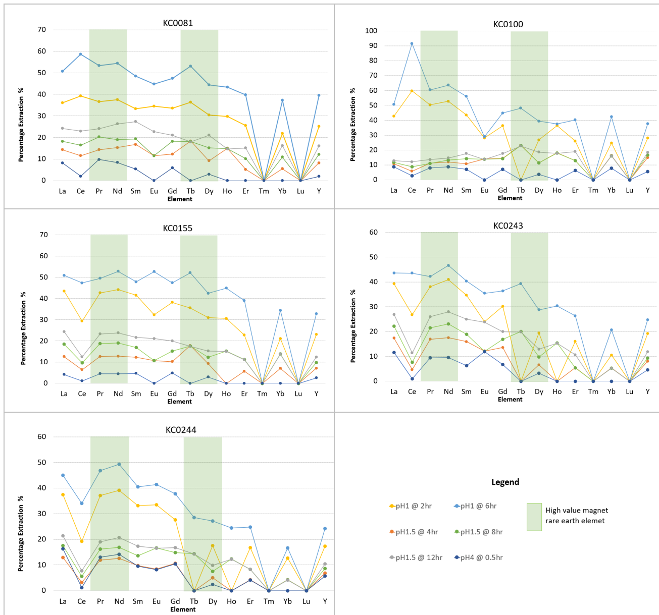
Figure 2: Extraction of rare earth elements using various diagnostic tests
