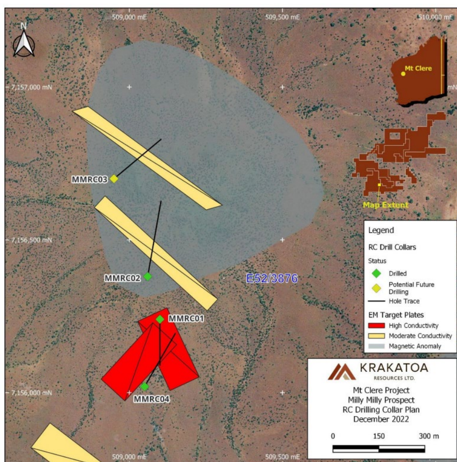
Figure 6: Drillhole plan showing location of the three drillholes completed at the Milly Milly target
