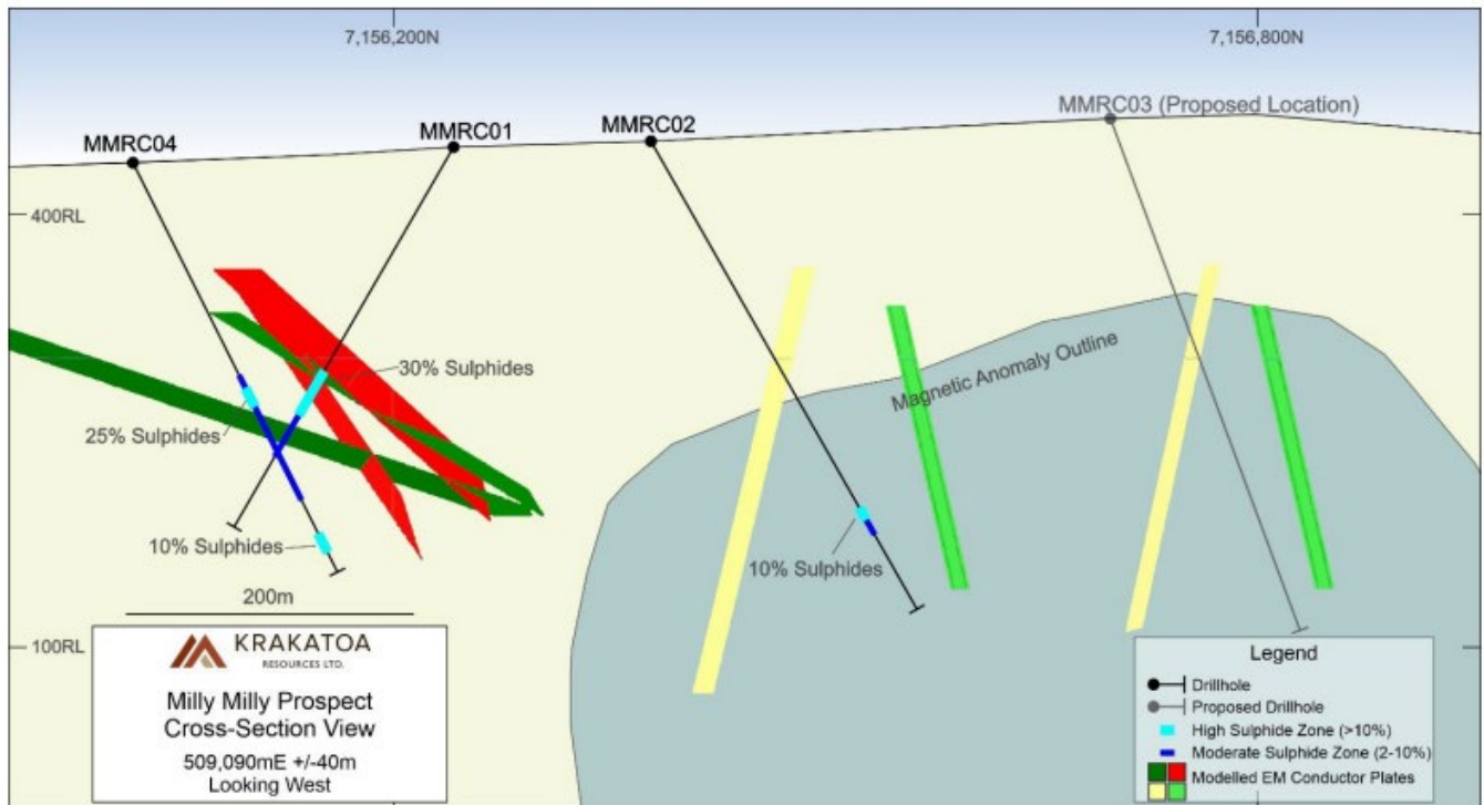
Figure 7: Section through MM-1 looking west, showing sulphide zones and relation to modelled EM plates (partially off-section)
