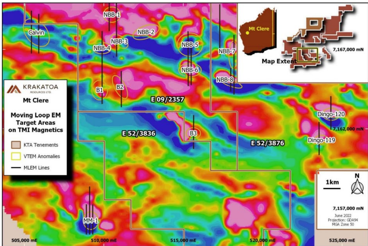
Figure 4: Map of Southern Cluster AEM targets showing MLEM lines over TMI magnetics
