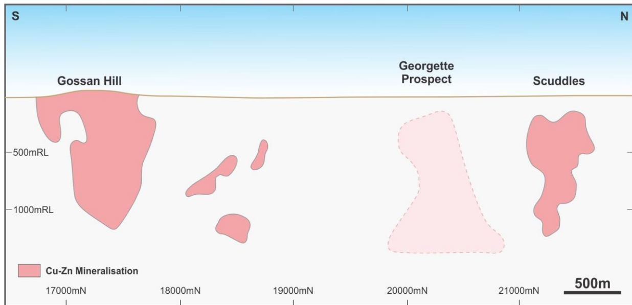
Figure 3a: Simplified Longitudinal Section of Gossan Hill and Scuddles (Golden Grove) VHMS Camp (modified after Hollis, S.P. et al (2017). VMS Mineralisation in the Yilgarn Craton, Western Australia: A Review of Known Deposits and Prospectivity Analysis of Felsic Volcanic Rocks. GSWA Report 165, p15)
