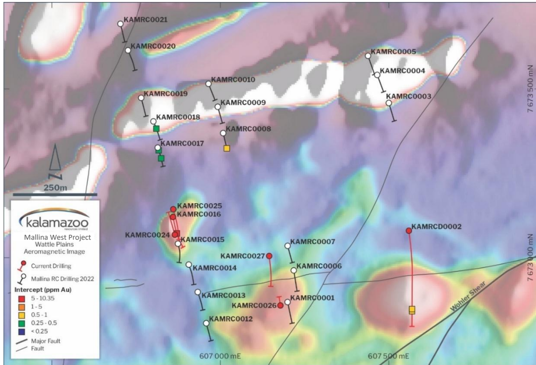
Figure 3: Wattle Plains Prospect 2024 and 2022 RC drilling programs with significant results on background aeromagnetic (TMI) image
