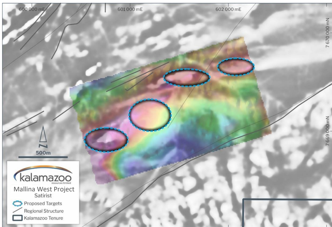
Figure 6: Satirist Prospect: Image of coincident and discrete gravity (colour overlay; detrended 1st Order Bouguer image) and aeromagnetic (underlying greyscale; RTP image) anomalies 4
