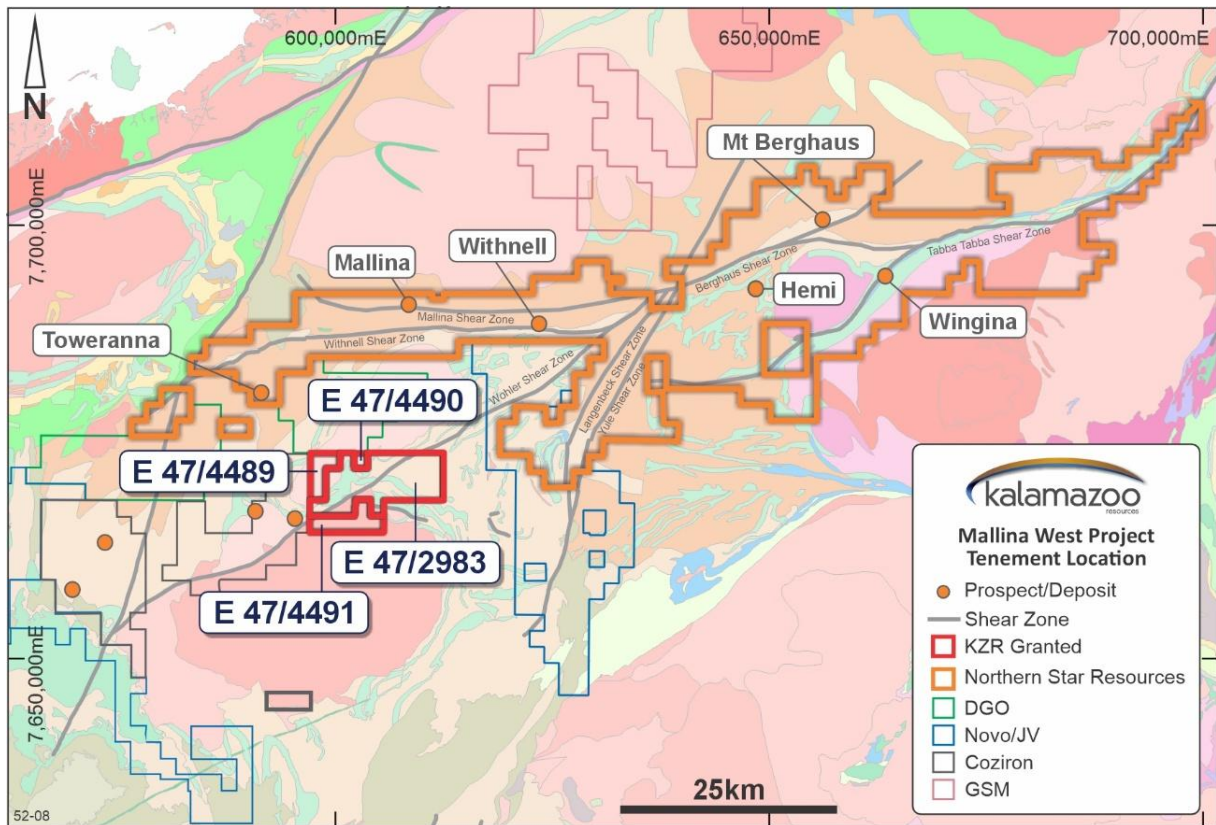
Figure 1: Mallina West Gold Project Tenement Location on background regional geology
