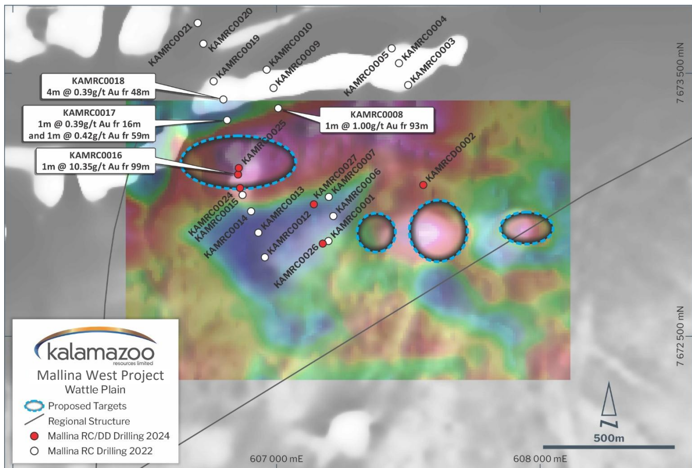
Figure 5: Combined 3D magnetic and gravity image and 2022 RC gold drilling results
