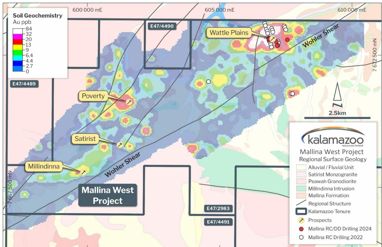
Figure 2: Mallina West gold prospects, Wohler Shear structure and gold in soil geochemistry
