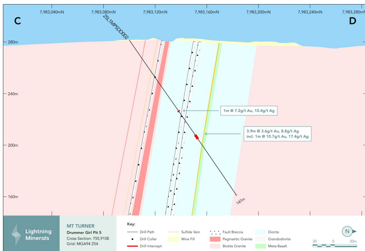
Figure 1: Cross-section of Hole 25L1MP5DD002 (Drummer Girl - Pit 5)
