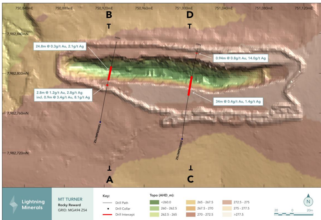
Figure 3: Plan view of Holes 25L1MP6DD001 and 25L1MP6DD002 (Pit 6 - Rocky Reward)
