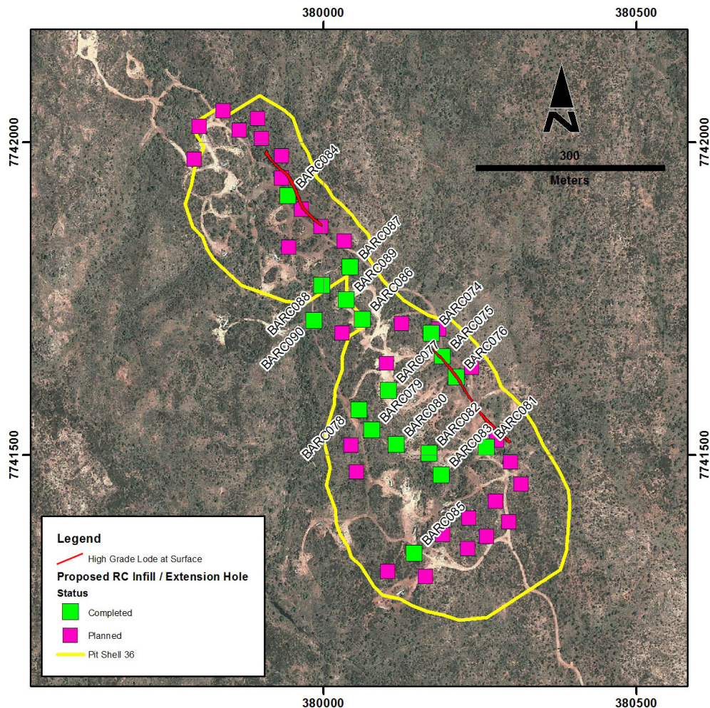
Figure 3 – Plan showing proposed in-fill RC & extension drilling
