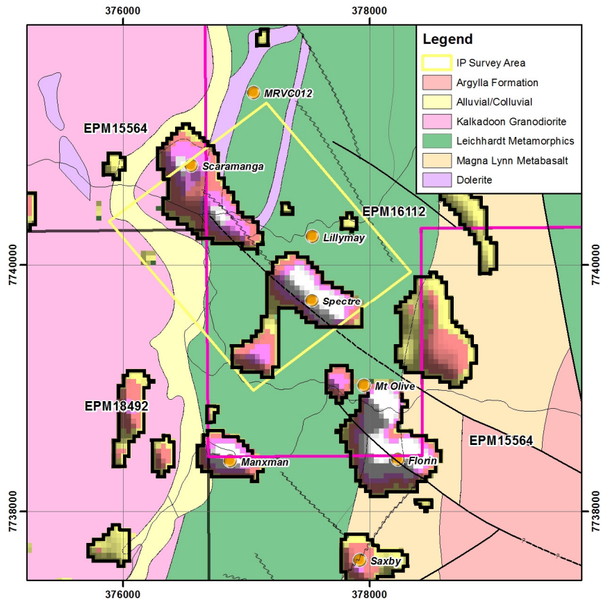
Figure 4 – Plan Showing IP Survey Area over Cu-in-soil geochemistry
