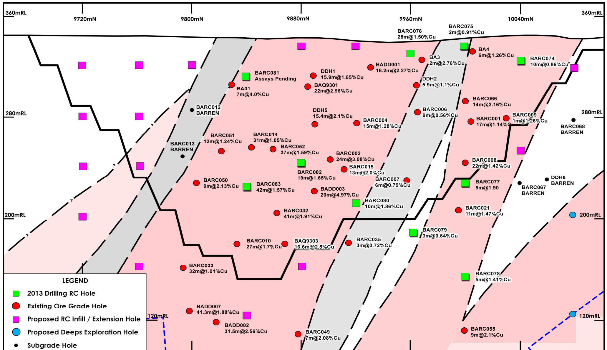
Figure 2 – Long Section showing recent drilling results and proposed in-fill RC & extension drilling
