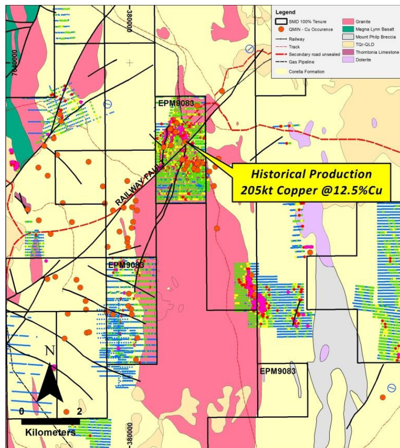
Figure 1 – Southern Hub Duchess soil geochemistry
