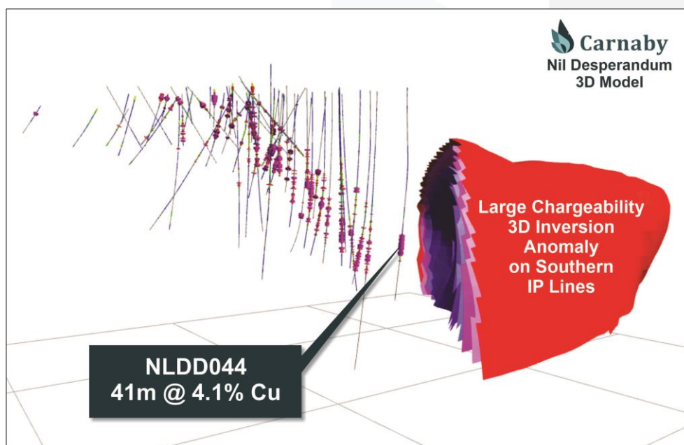
Figure 5#. Nil Desperandum 3D IP chargeability inversion model looking southeast.
