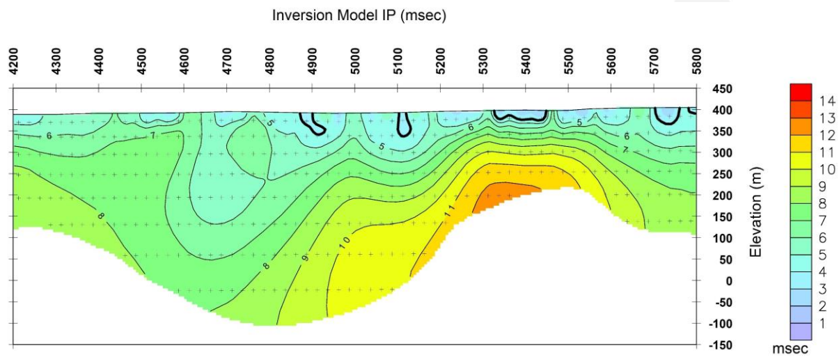
Figure 6. IP line L18500N Inversion Model Chargeability Section.
