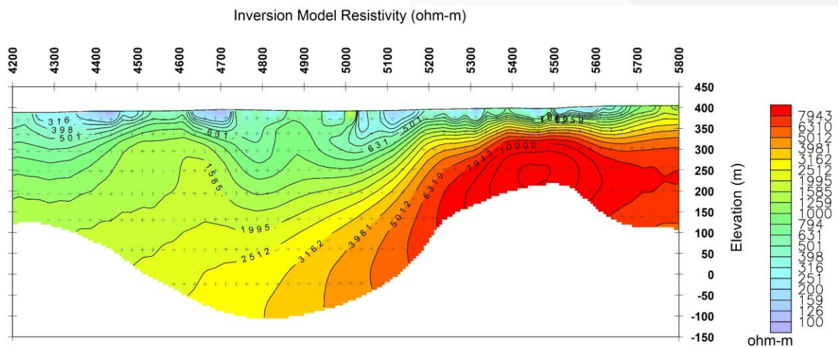
Figure 7. IP line L18500N Inversion Model Resistivity Section.
