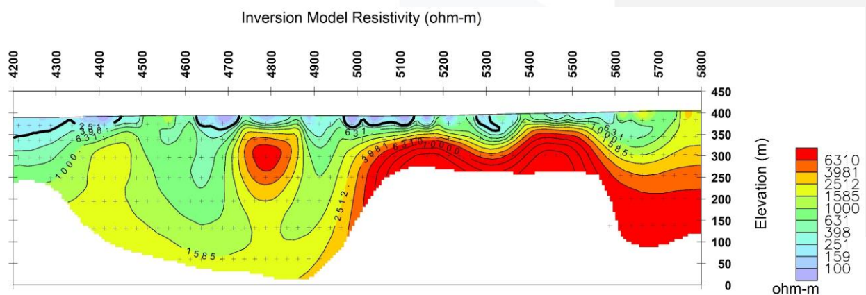
Figure 7. IP line L18600N Inversion Model Resistivity Section.
