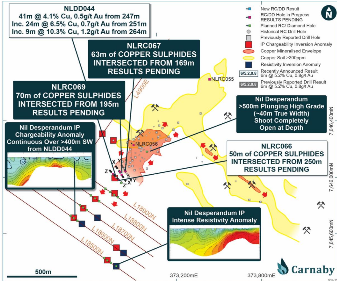
Figure 1. Plan of Nil Desperandum Showing location of NLRC067, NLRC069 and IP.
