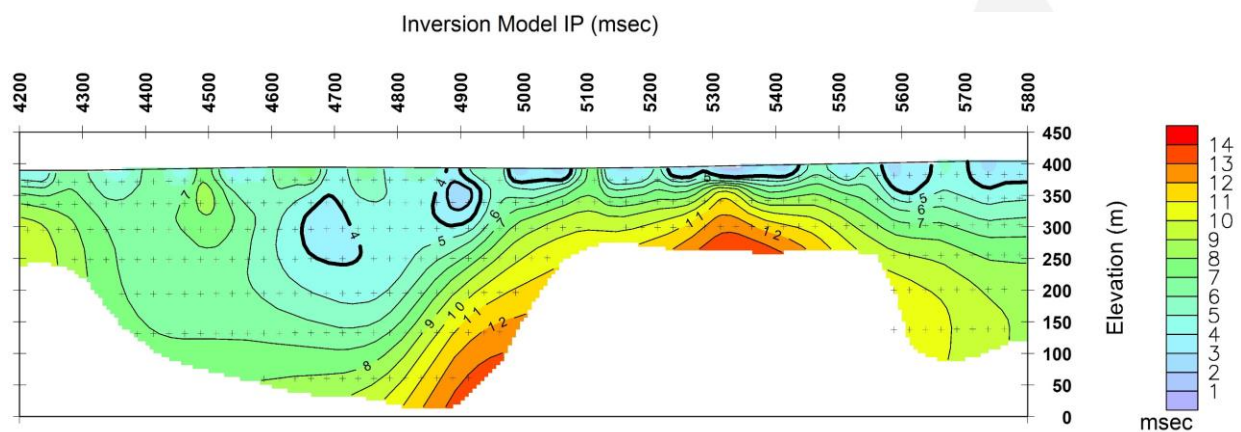
Figure 6. IP line L18600N Inversion Model Chargeability Section.
