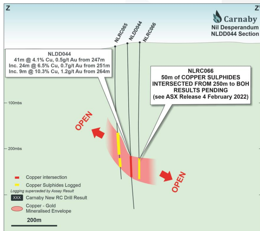
Figure 3. Drill Section showing location of drill hole NLDD044 and NLRC066.
