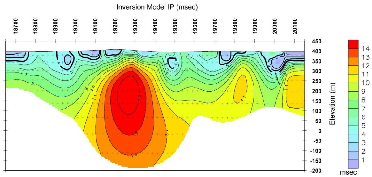
Figure 6. IP line L4900E Inversion Model Chargeability Section.
