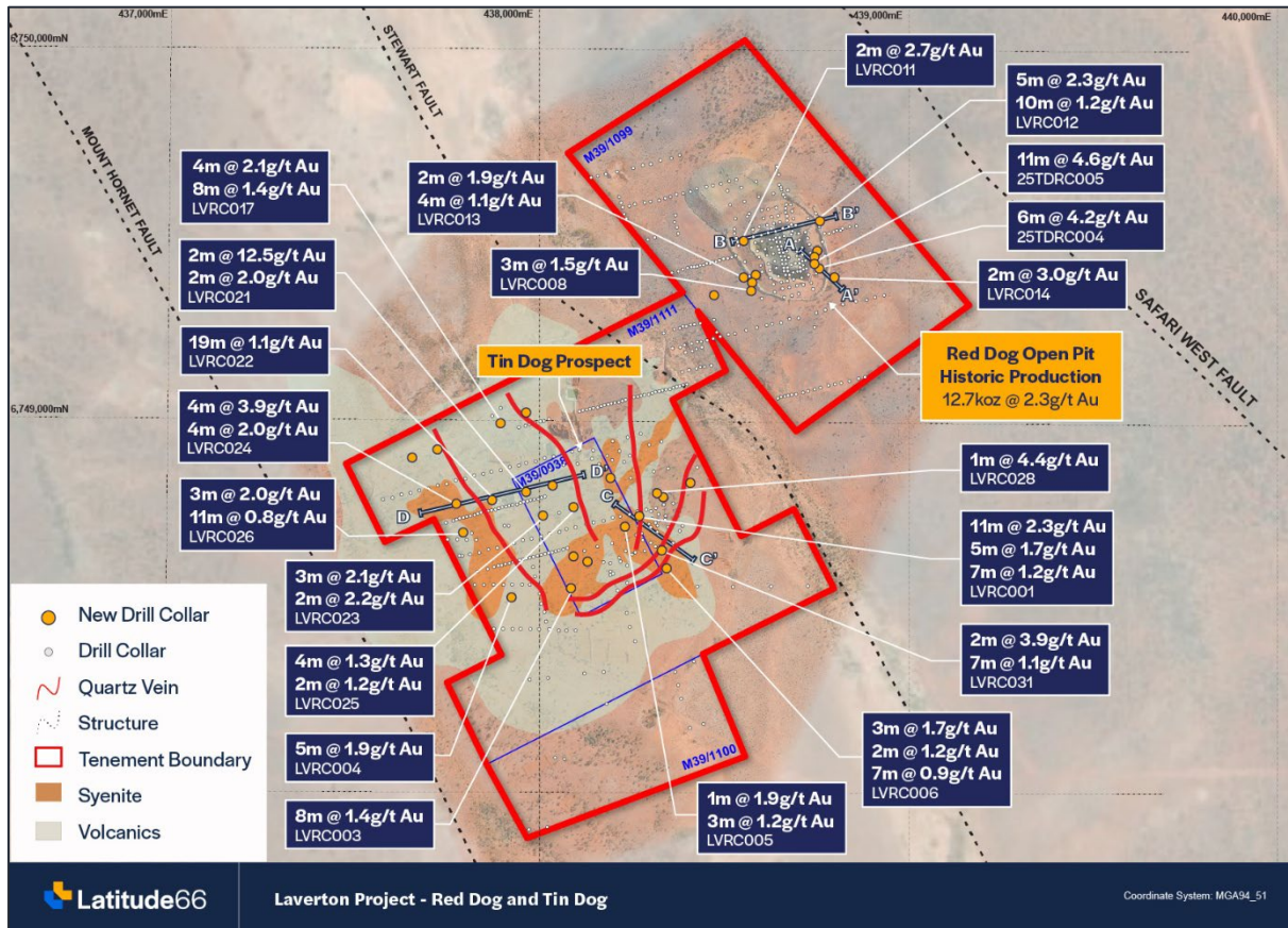
Figure 1: Plan view of the Red Dog and Tin Dog Prospects with significant intersections
