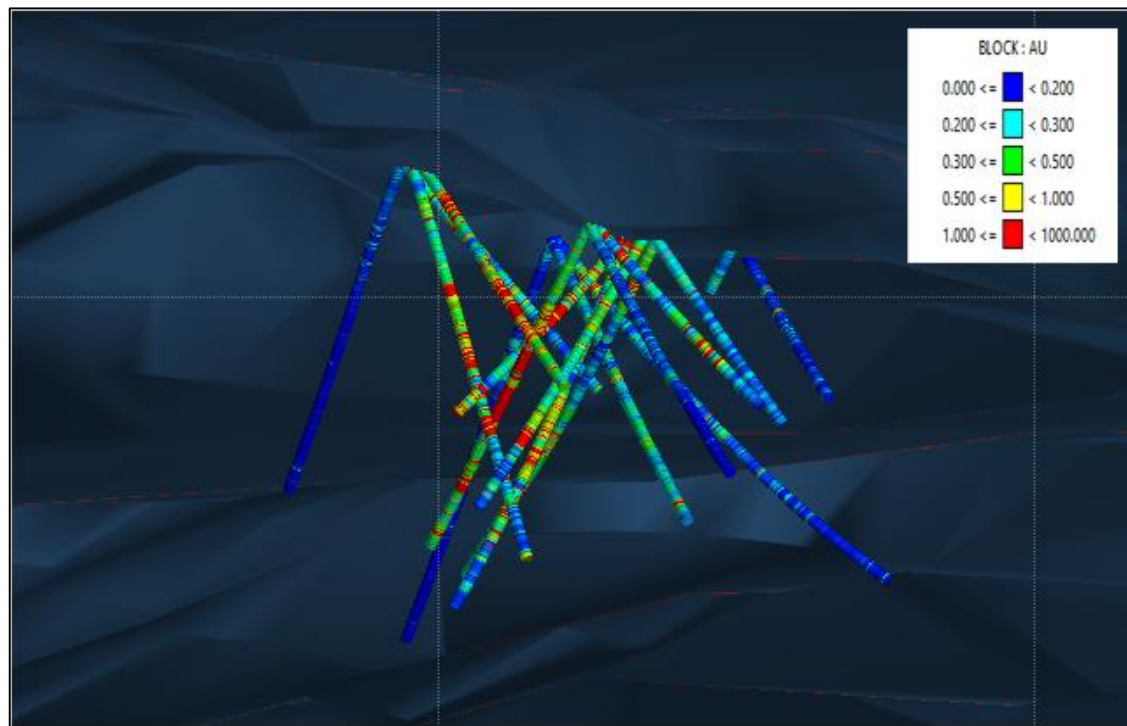
Isometric View Dosquibradas Drilling – Not to Scale
