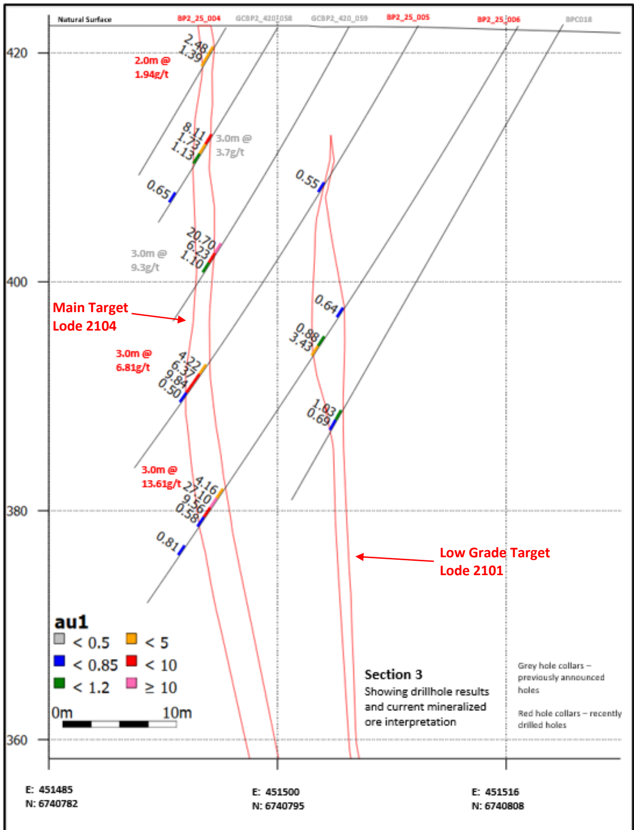
Figure 5. Cross Section 3 of High-Grade Intersection in Blue Peter 2
