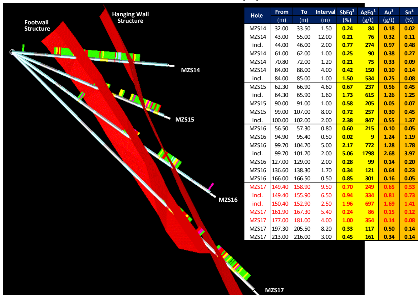
Figure 3. Montezuma Antimony & Silver Project - Cross Section 5364090N (looking North) showing SbEq & AgEq intercepts plus gold (Au) and tin (Sn) intercepts in drill holes MZS14 to MZS17. Three of the five mineralised zones from drill hole MZS17 used for the bulk scenario in Table 4 are highlighted in red.
