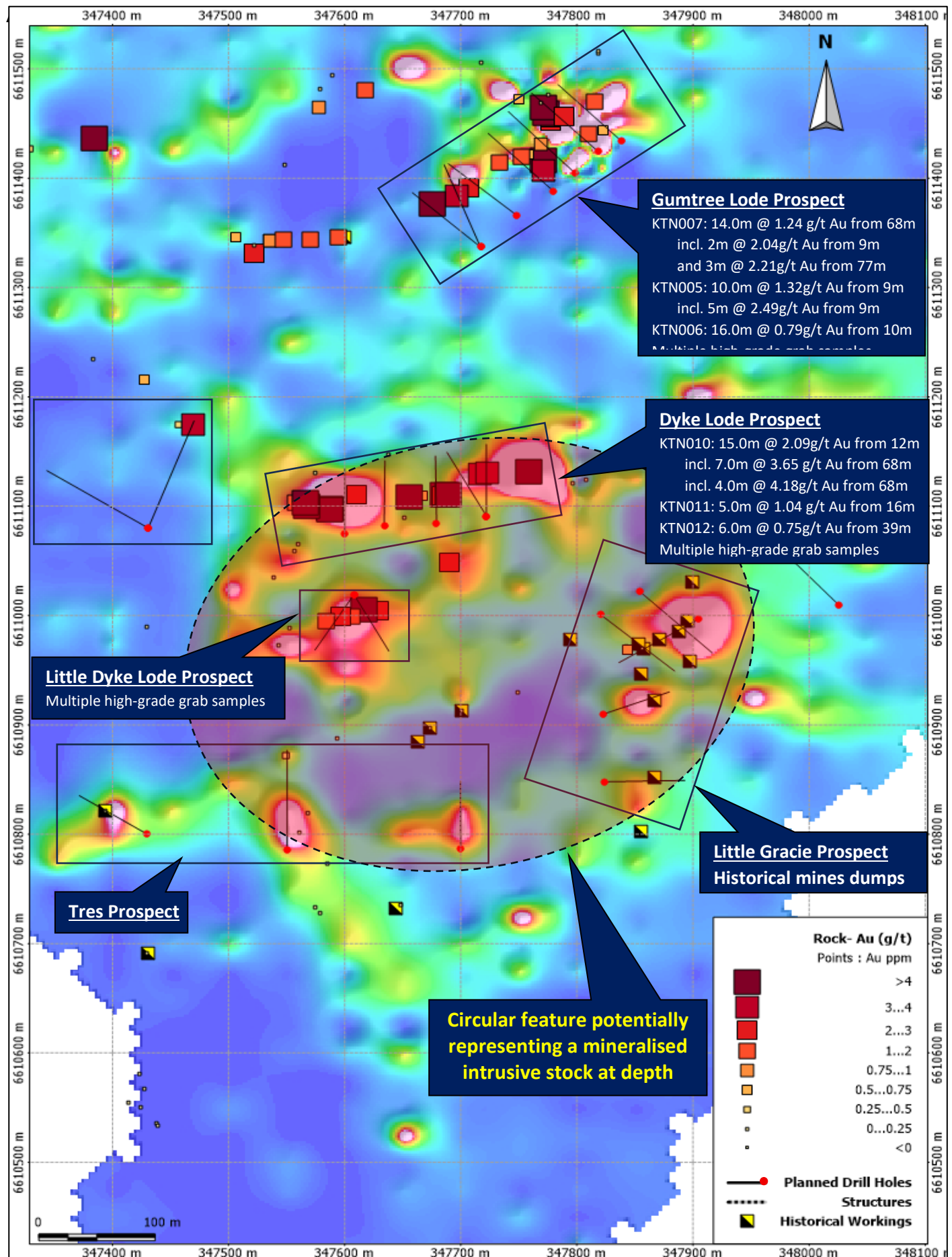
Figure 3. Uralla Gold Project - planned drilling, deep soil gold assay image (1,192 auger holes) and previously reported drill and grab sample results 1-10
