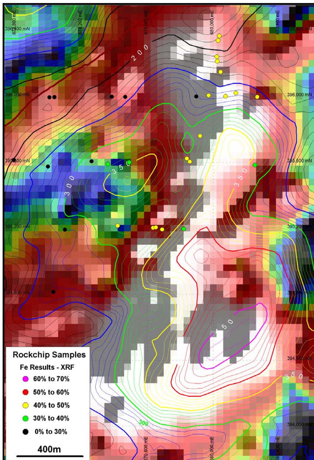
Figure 3: Logmangan Prospect – Rockchip Sample Results (Iron) on Aeromagnetic Image (Analytical Signal of Total Magnetic Intensity)
