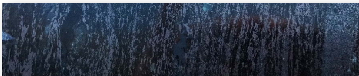
Polished magnetite gneiss core sample from drillhole NESD011
