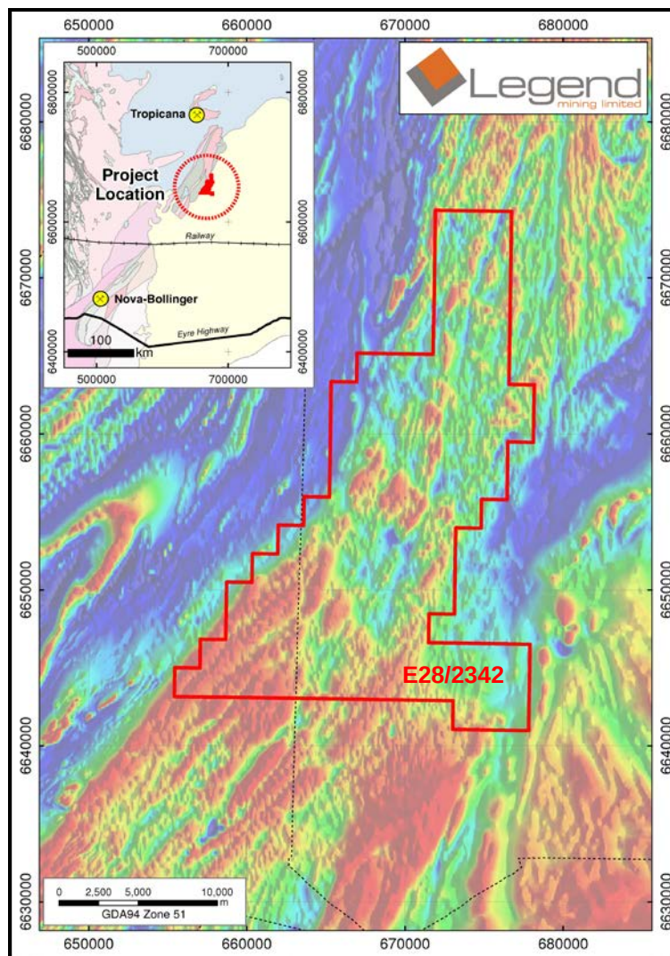
Figure 4: Tenement Application E28/2342 Over Aeromagnetic Image
