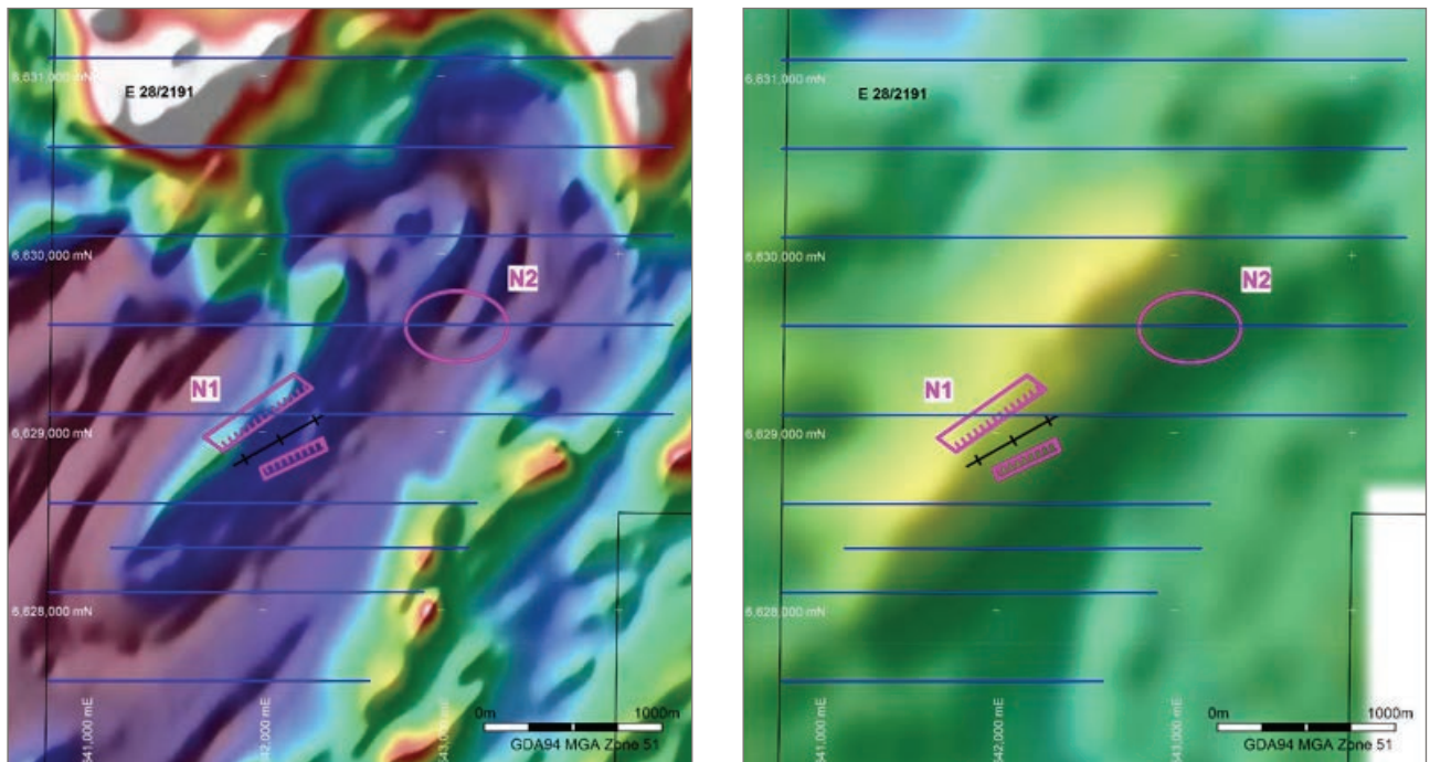
Figure 4: Area N Conductors on Aeromagnetic (left) and Gravity (right) Images
