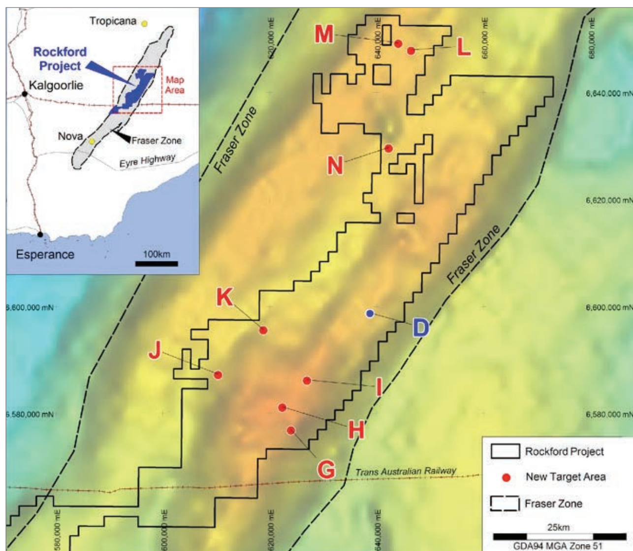
Figure 3: Rockford Project Target Areas on Regional Gravity
