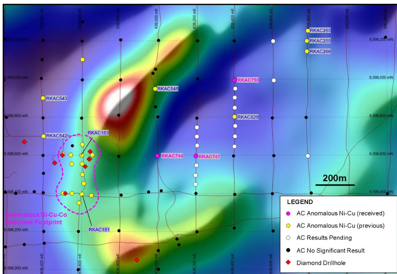
Figure 4: Summary of Anomalous Ni-Cu Aircore Results at Mawson
