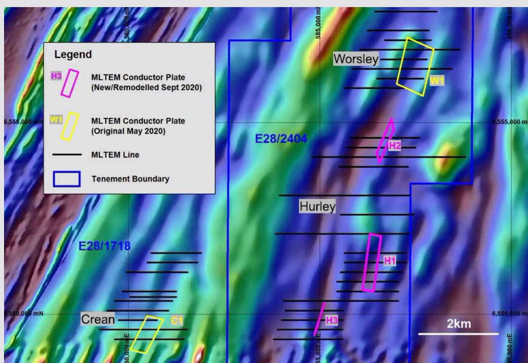
FIGURE 14: MLTEM SURVEY OVER HURLEY, WORSLEY AND CREAN PROSPECTS
