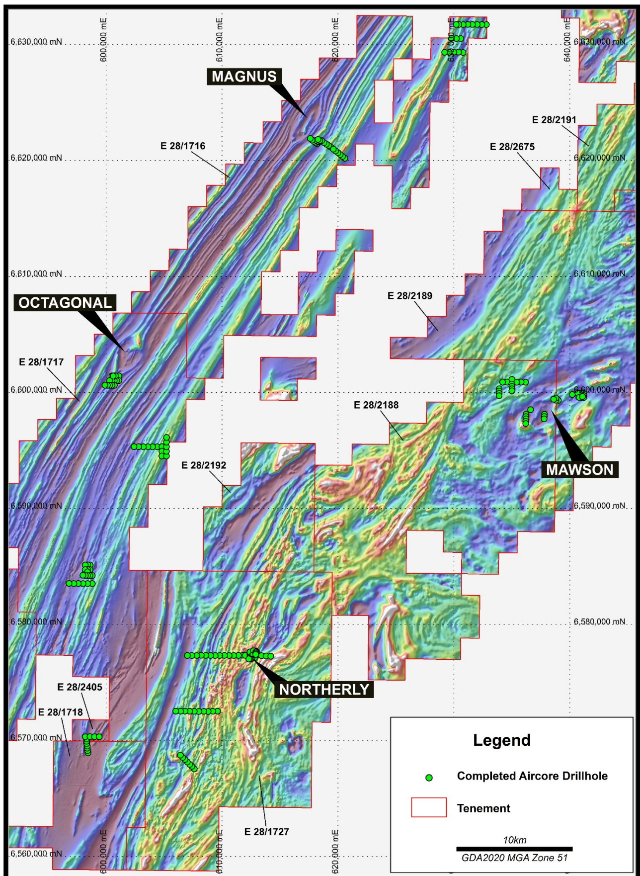
Figure 5: Regional aircore drilling completed over aeromagnetics
