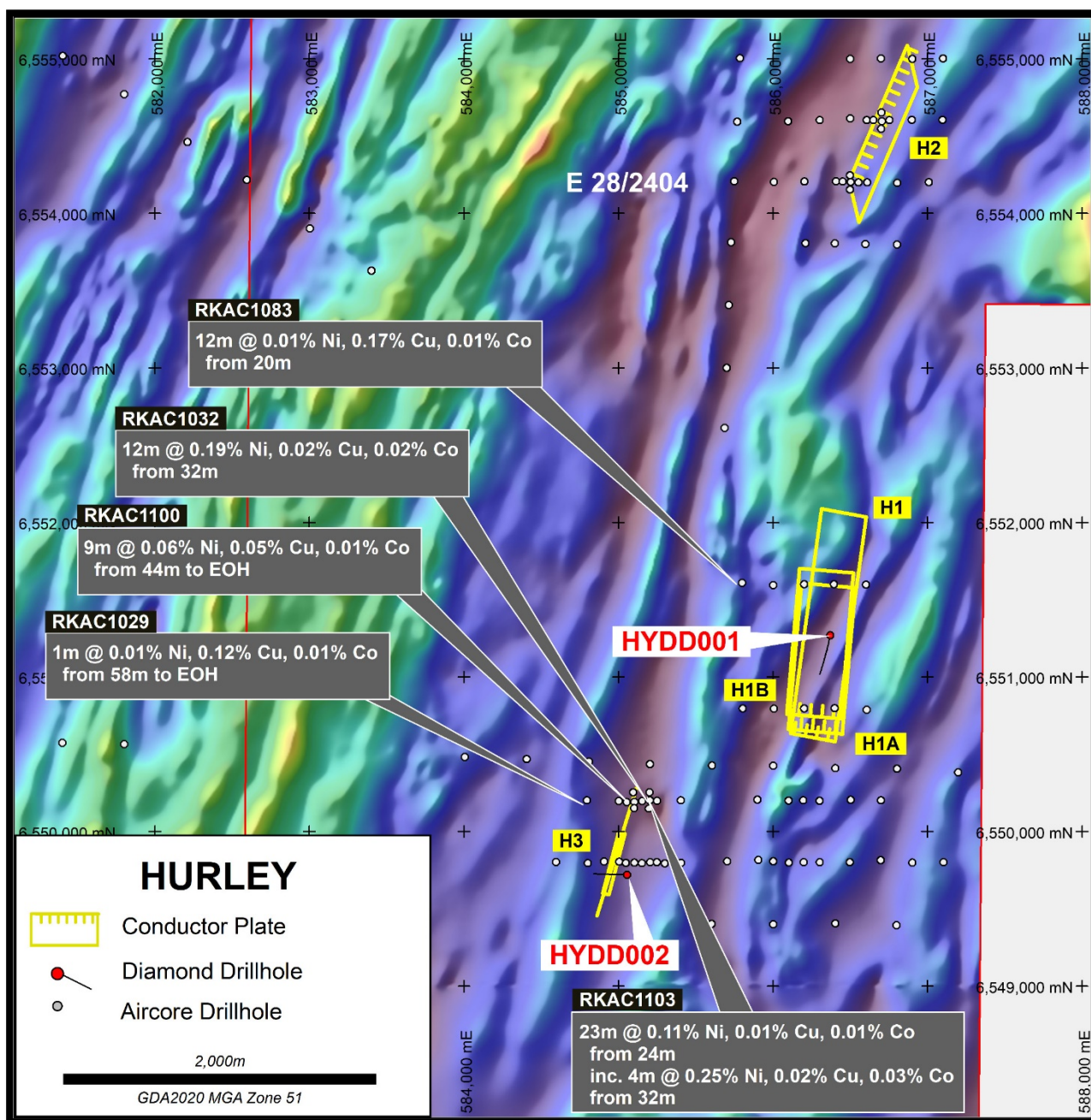
Figure 3: Hurley Prospect showing drilling completed over aeromagnetics
