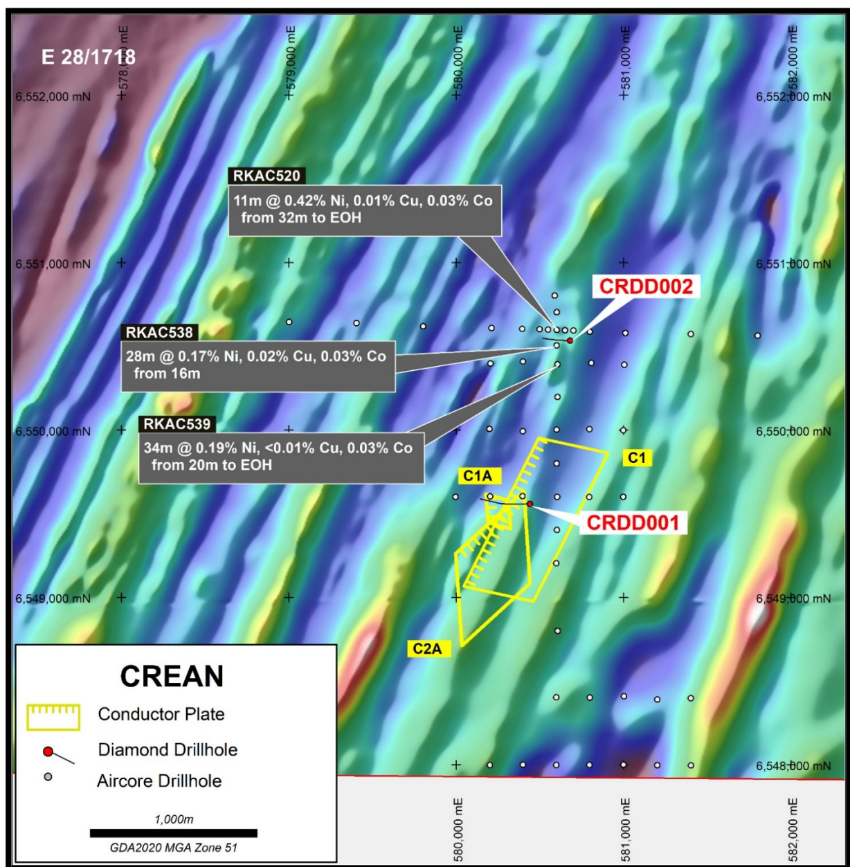
Figure 2: Crean Prospect showing drilling completed over aeromagnetics
