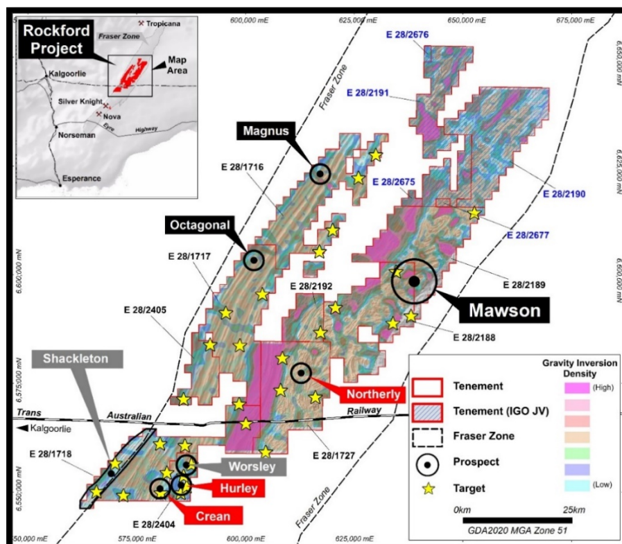
Figure 1: Regional Prospect Locations on Aeromagnetics
