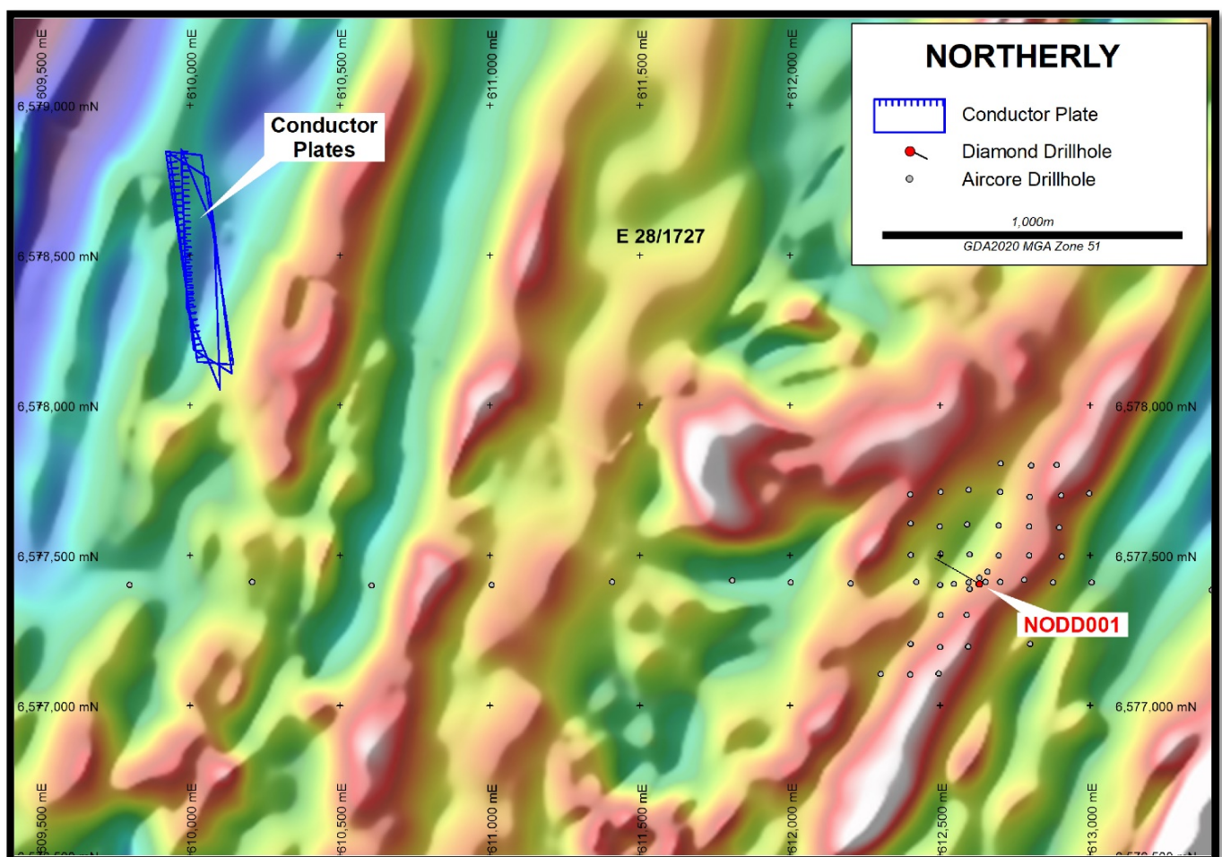
Figure 4: Northerly Prospect showing completed aircore drilling and the N1 MLTEM conductor over aeromagnetics
