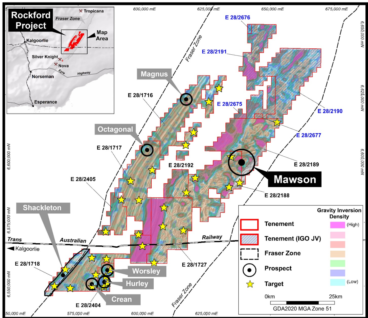
Figure 6: Rockford Project – Mawson Location
