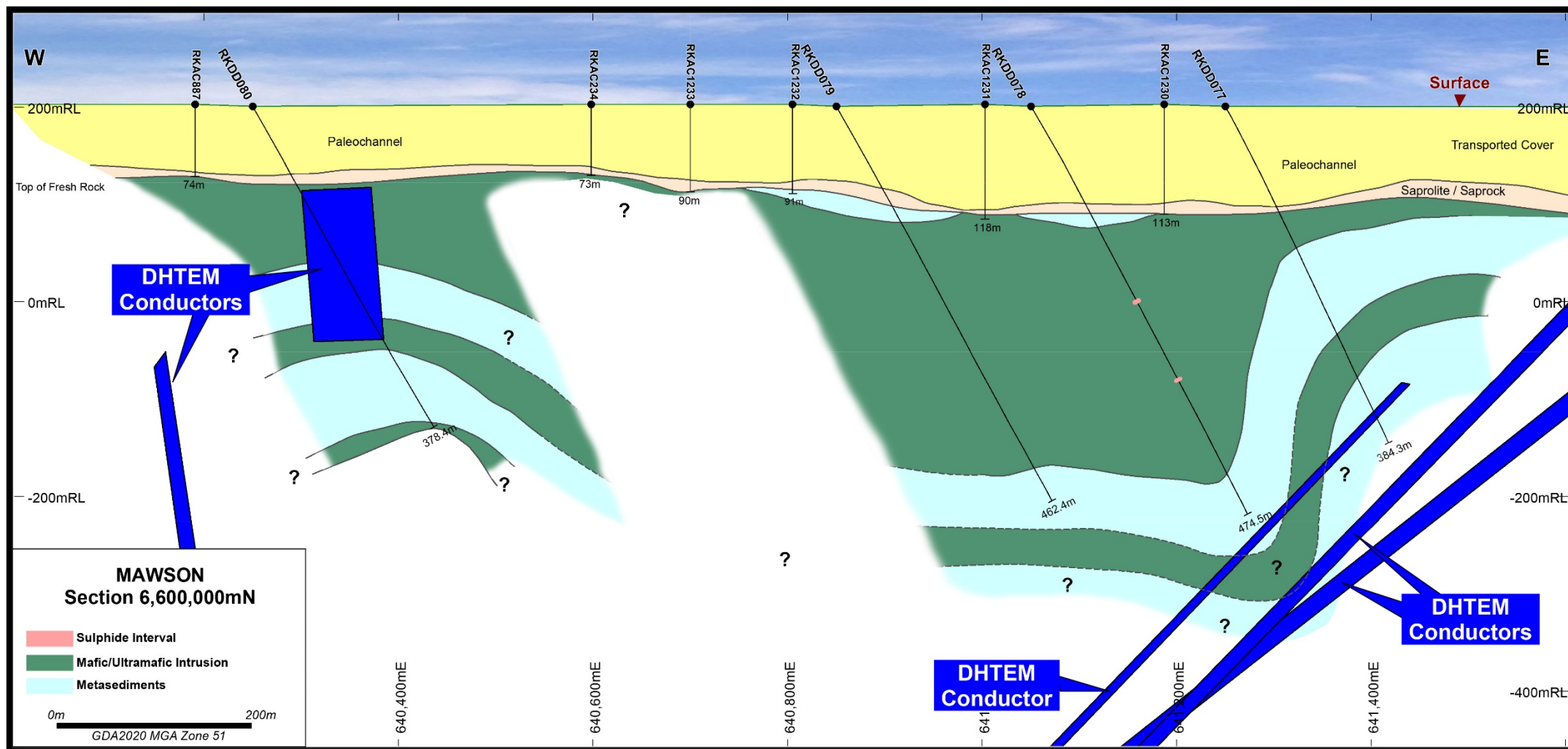
Figure 4: Drill section 6,600,000mN looking north
