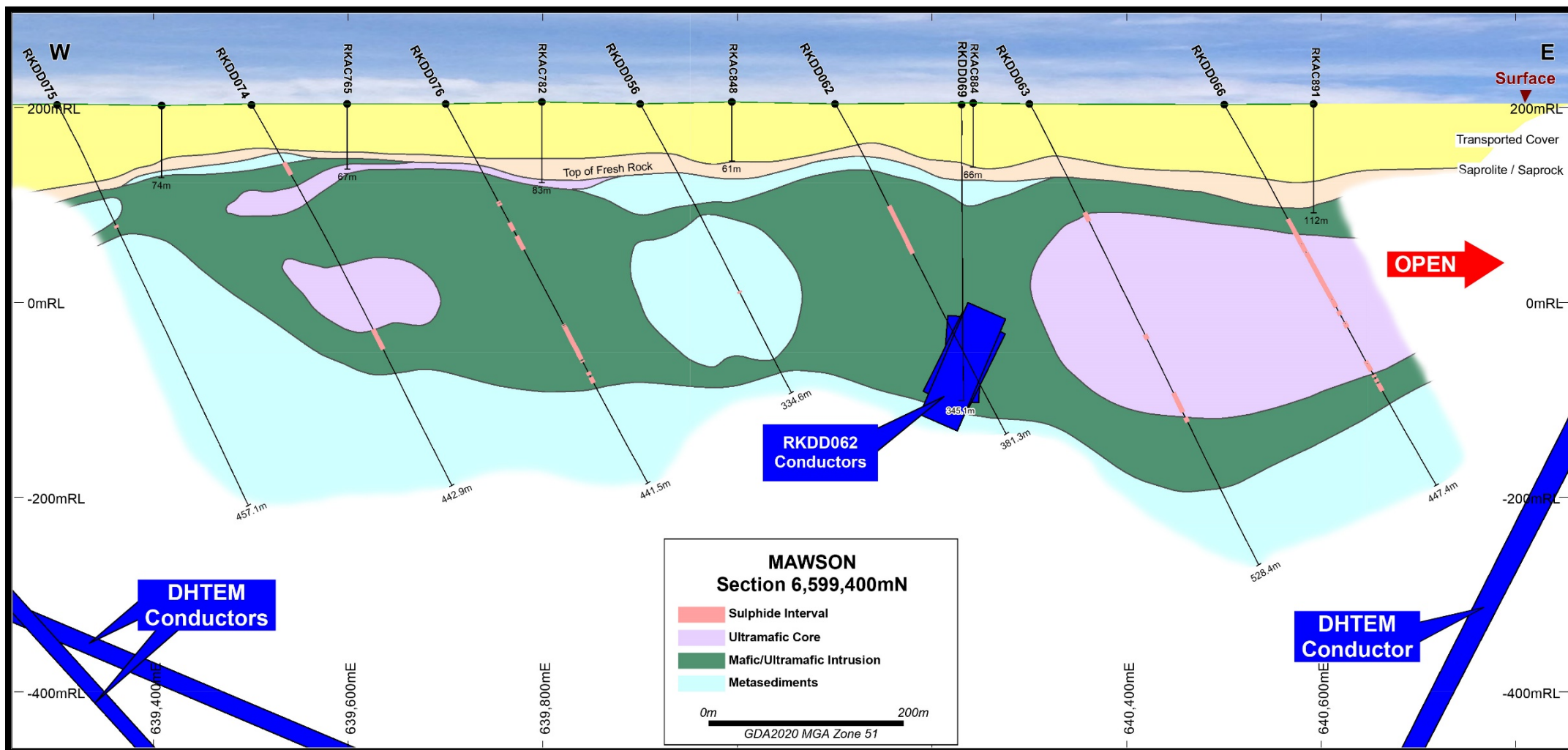
Figure 2: Drill section 6,599,400mN looking north
