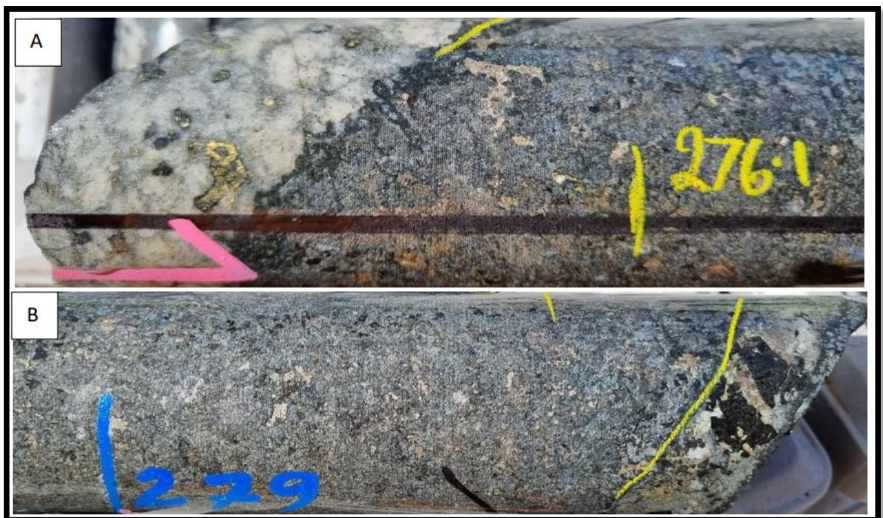
Photo 1: Ni-Cu sulphide mineralisation from RKDD074 from 276-279m
