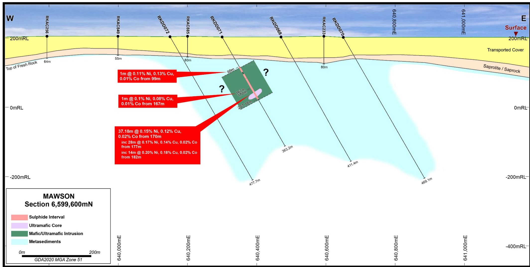
Figure 3: Drill section 6,599,600mN looking north
