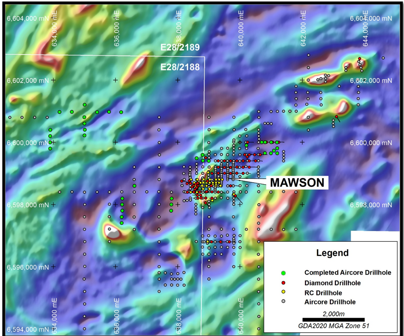
Figure 5: Mawson Intrusive Complex Proposed Aircore Drilling
