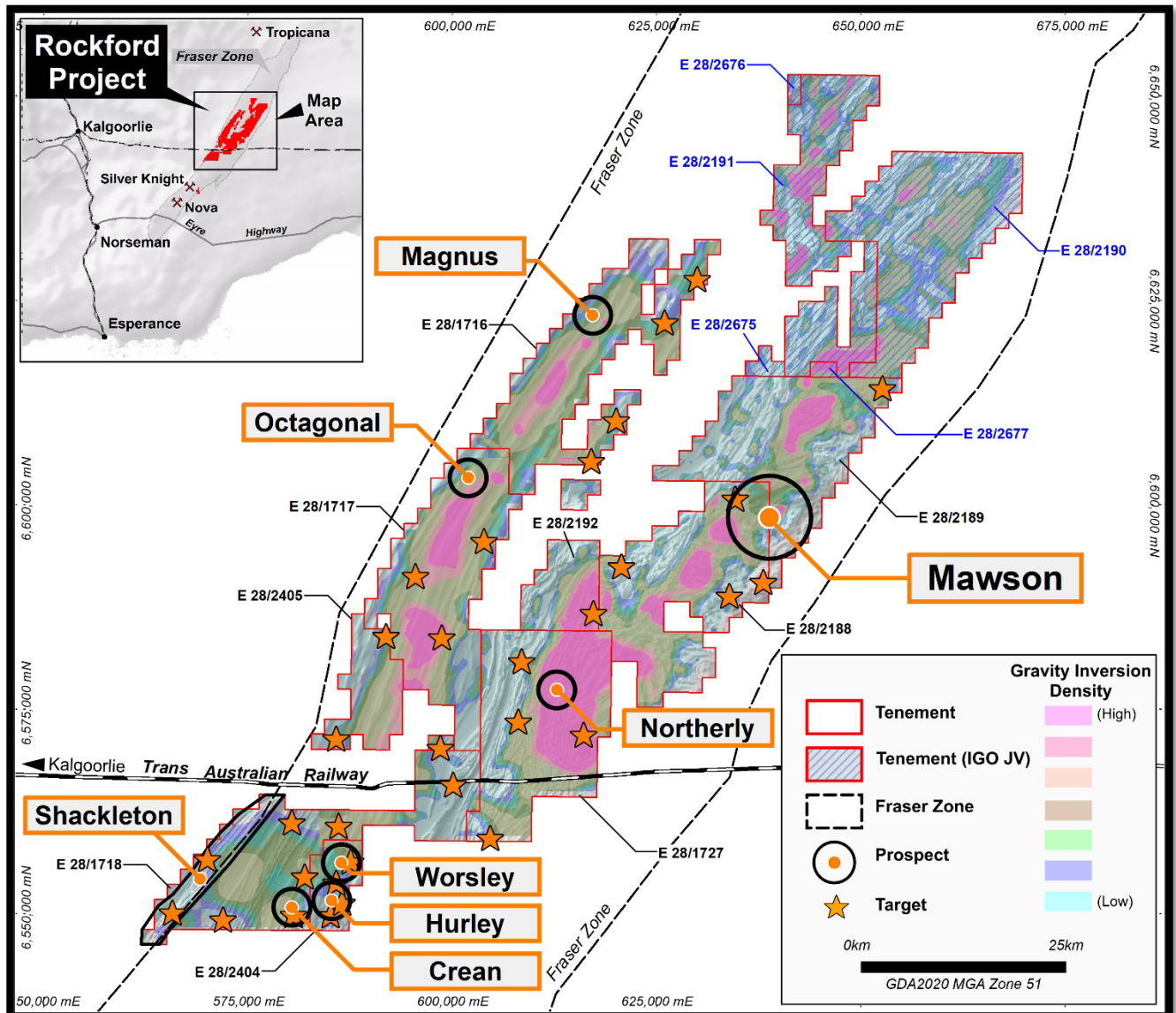
Figure 6: Rockford Project Prospect Locations on Gravity
