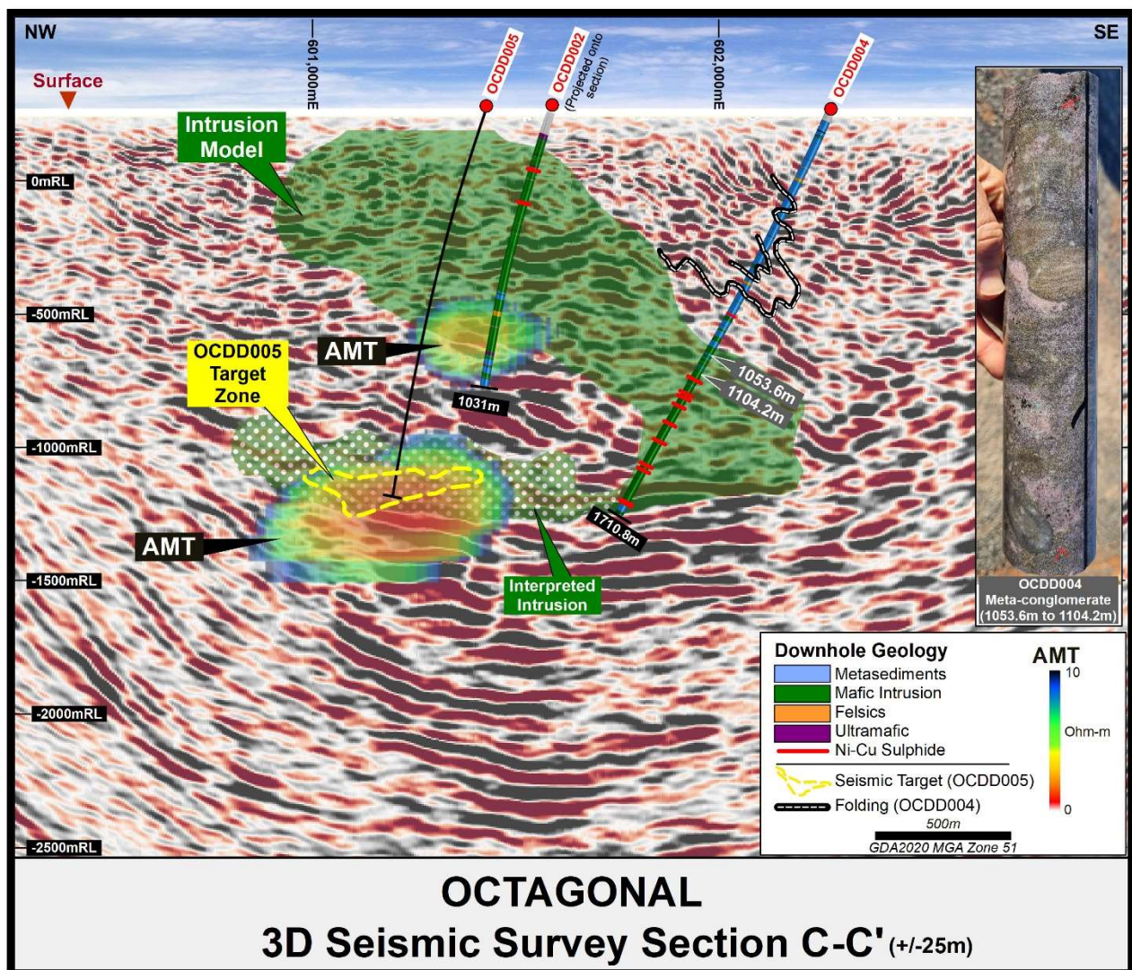
Figure 2: Section C-C' showing drillholes OCDD002, OCDD004 and OCDD005 (ongoing) on seismic section and downhole geology and structure, the Octagonal intrusion and interpreted intrusion, and primary seismic and AMT targets.
