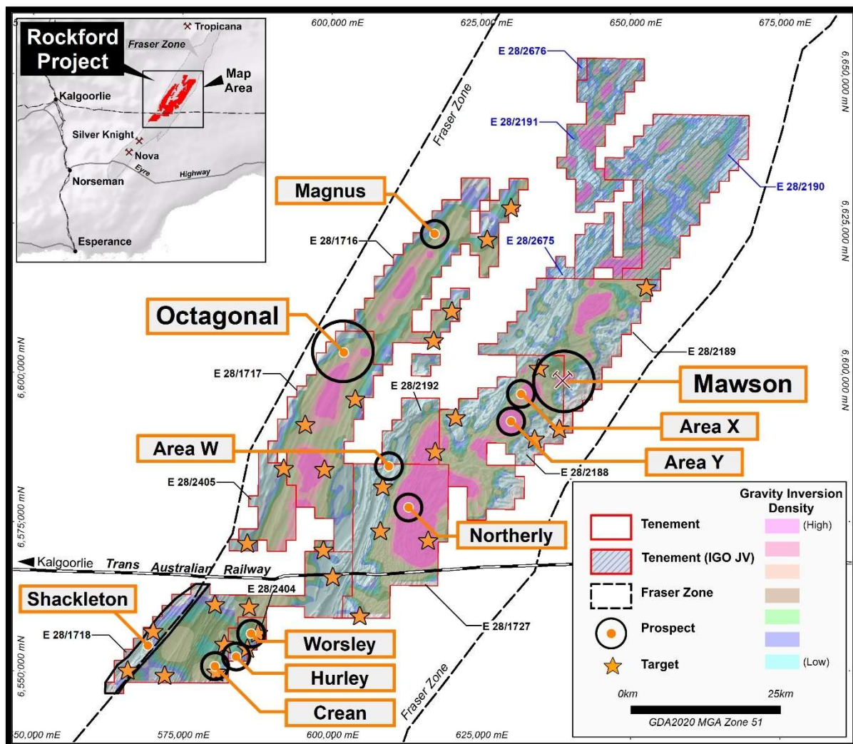
Figure 3: Rockford Project Prospect Locations on Gravity.
