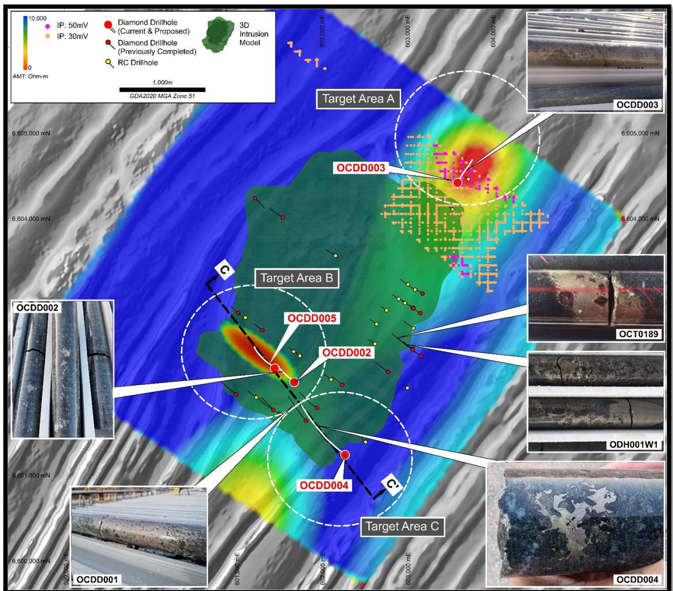
Figure 1: Priority target areas and diamond drillholes shown with Octagonal intrusion model, IP anomalies, 2D & 3D AMT anomalies, and visual Ni-Cu mineralisation on AMAG.
