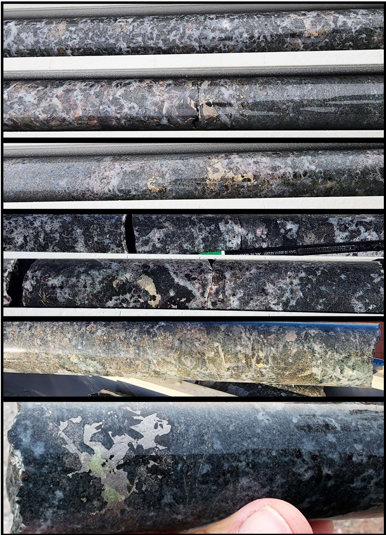
Photo 2: Blebbly and disseminated Ni-Cu sulphide intervals from 1195m to 1496m in fertile troctolite, olivine gabbro, and pyroxenite in diamond drillhole OCDD004
