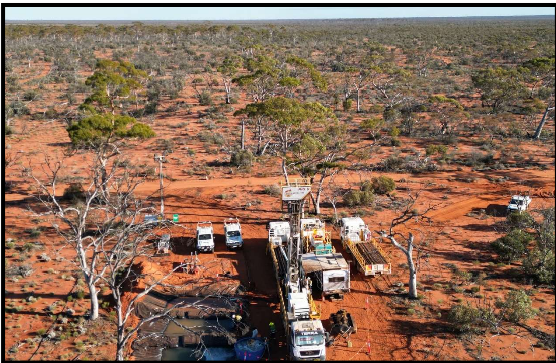
Photo 1: Diamond drillhole OCDD005 underway at Target Area B.
