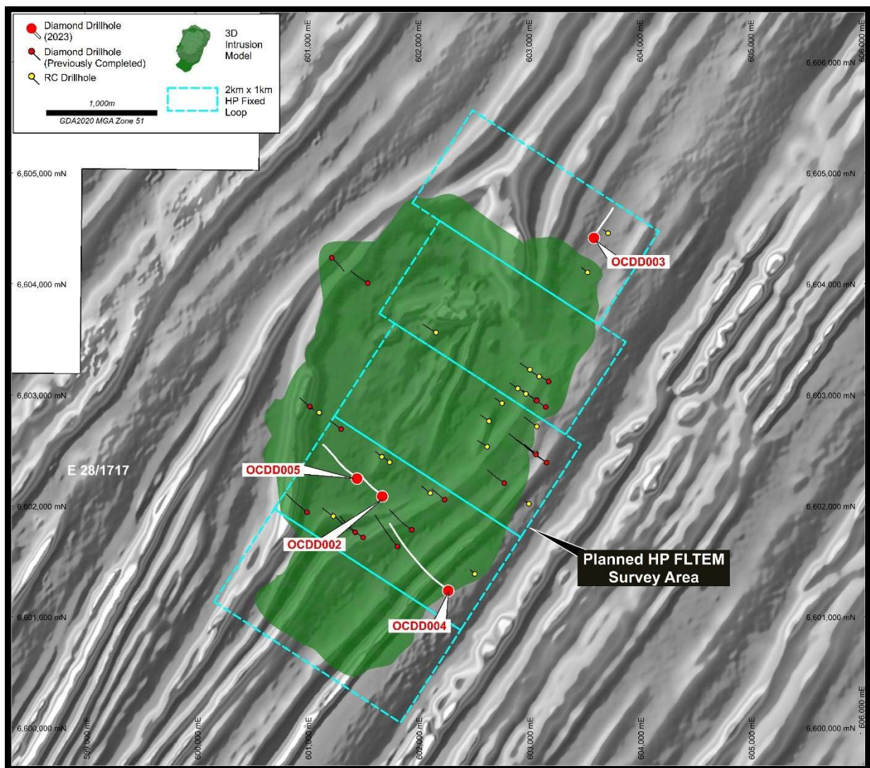
Figure 1: Octagonal plan view showing proposed HPFLTEM survey loops and the interpreted Octagonal intrusion model projected to surface on AMAG.
