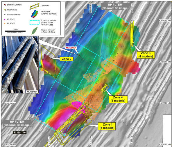
Magnus plan view showing completed HPFLTEM on AMAG See ASX announcement dated 16 October 2024 for full details
