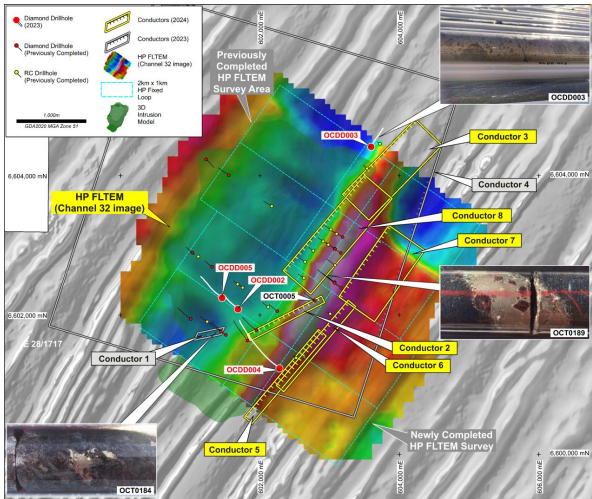
Octagonal plan view showing completed HPFLTEM on AMAG See ASX announcement dated 20 August 2024 for full details
