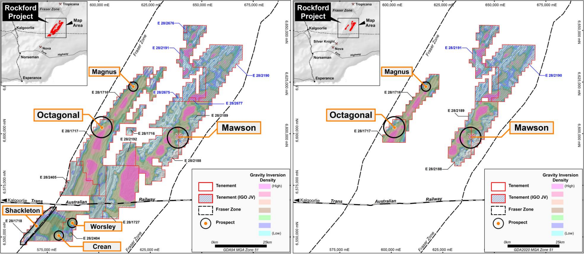
Rockford Project Prospect Locations on Gravity - 2019 +3,000km 2 (79% LEG Managed)
