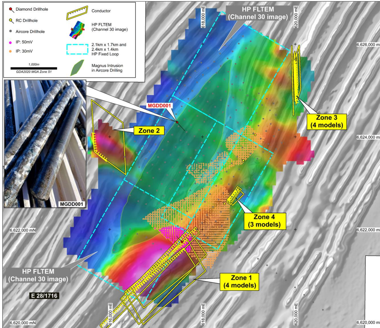
Magnus plan view showing completed HPFLTEM survey loops with identified conductors on channel 30HD imagery, IP anomalies, and the interpreted Magnus intrusion model projected to surface on AMAG. See ASX announcement dated 16 October 2024 for full details
