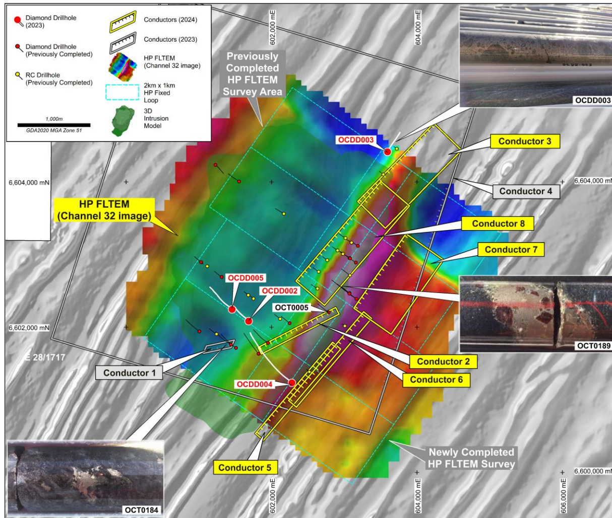
Octagonal plan view showing completed HPFLTEM survey loops with new and existing conductors on channel 32HD imagery with the interpreted Octagonal intrusion model projected to surface on AMAG. See ASX announcement dated 20 August 2024 for full details
