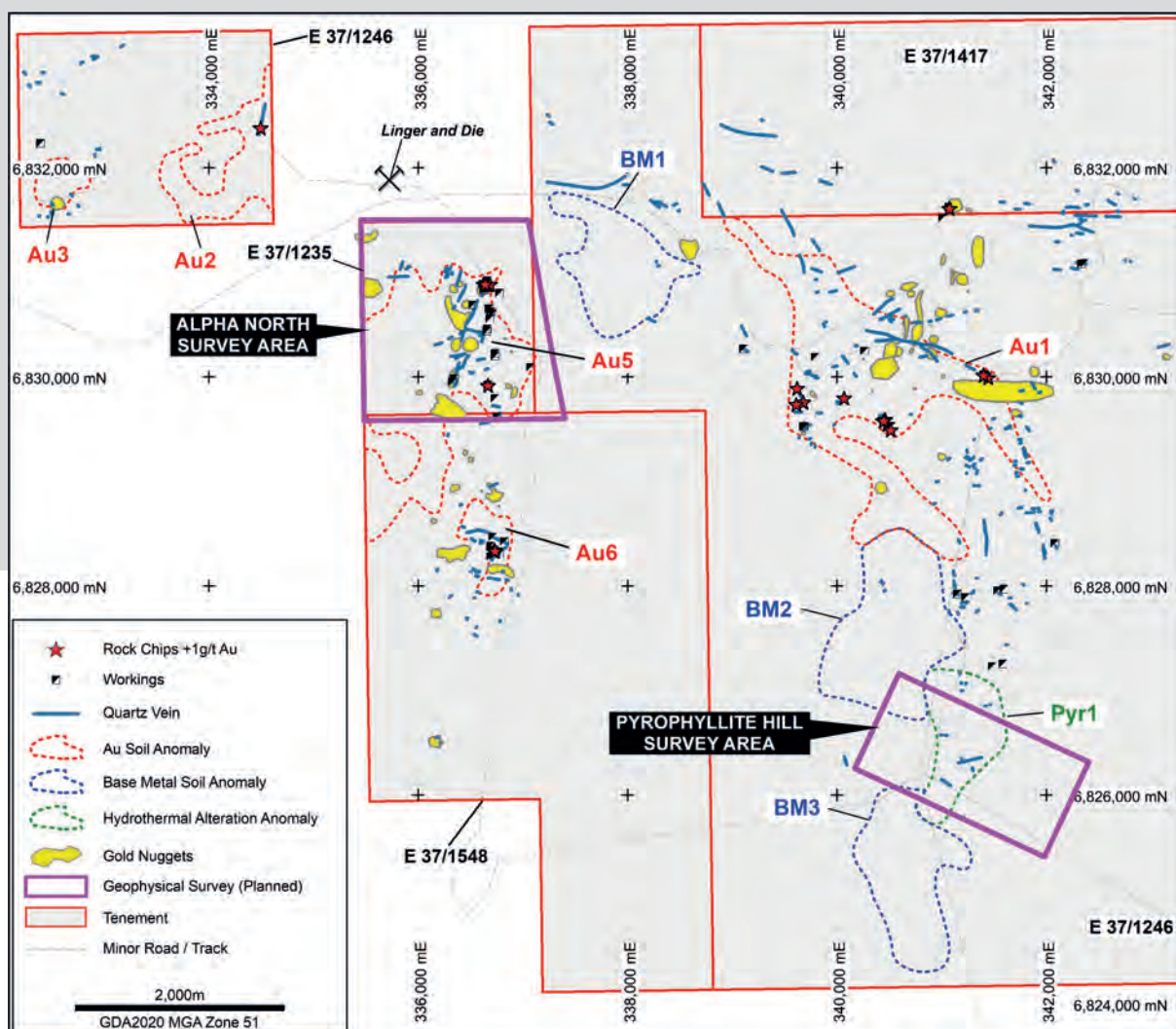
FIGURE 4 Pinnacle Well Project – Gold, base metal and hydrothermal alteration UFF soil anomalies, extensive quartz veining, gold workings, gold nugget patches, >1g/t Au rockchips with proposed geophysical survey areas
