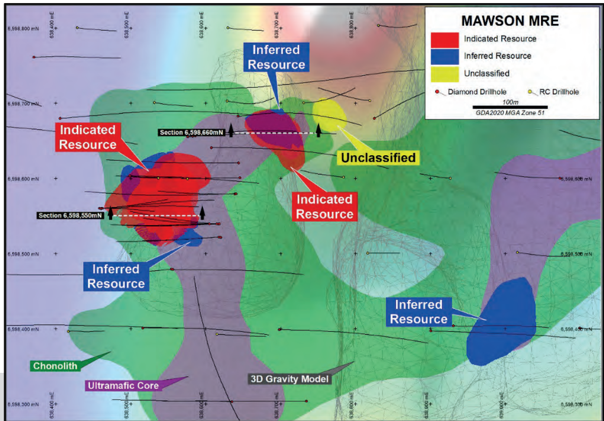
FIGURE 7 Mawson Mineral Resource Classification projected to surface with drillhole locations and chonolith projected to surface on Aeromagnetics
