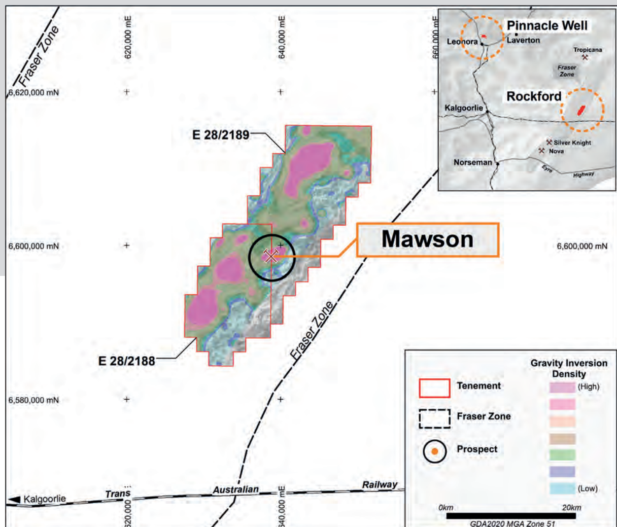
FIGURE 5 Rockford Project with Mawson location over regional gravity inversion
