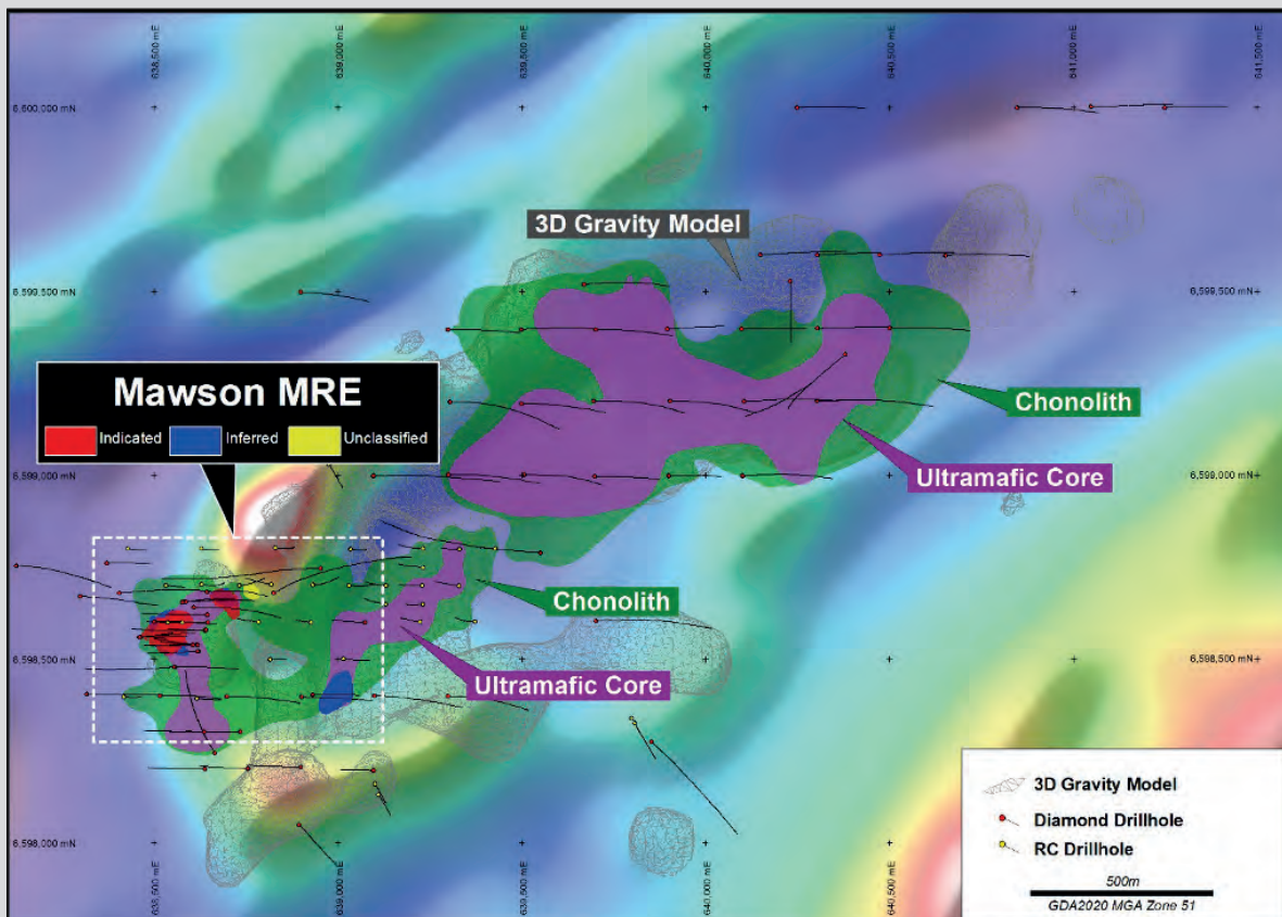
FIGURE 6 Mawson Intrusion and Mineral Resource Classification Area
