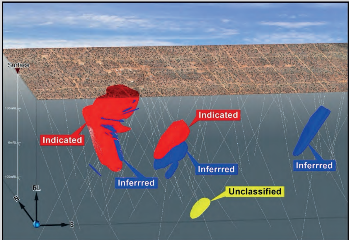
FIGURE 8 Mawson Mineral Resource Classification – oblique view facing north-west
