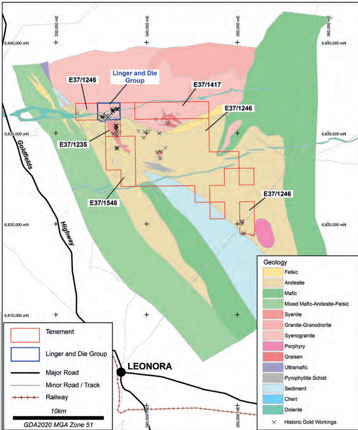
FIGURE 2 Pinnacle Well Project tenement locations on interpreted geology
