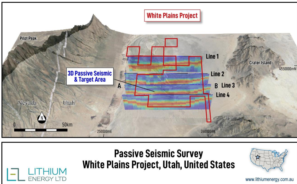
Figure 14: 3D passive seismic survey results from 4 survey lines within the White Plains claims area (shown in red)
