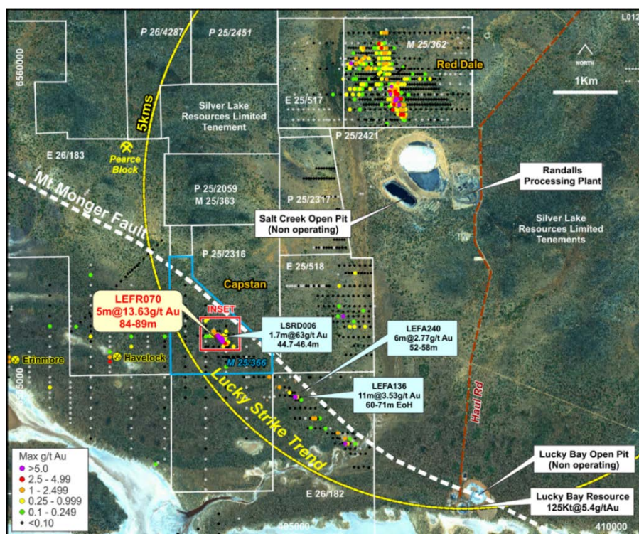
Figure 1 Location plan of Lefroy tenements, showing drill holes and the Lucky Strike, Red Dale and Capstan prospects proximal to the Randalls Processing plant. Refer to Figure 2 for detail on inset.
