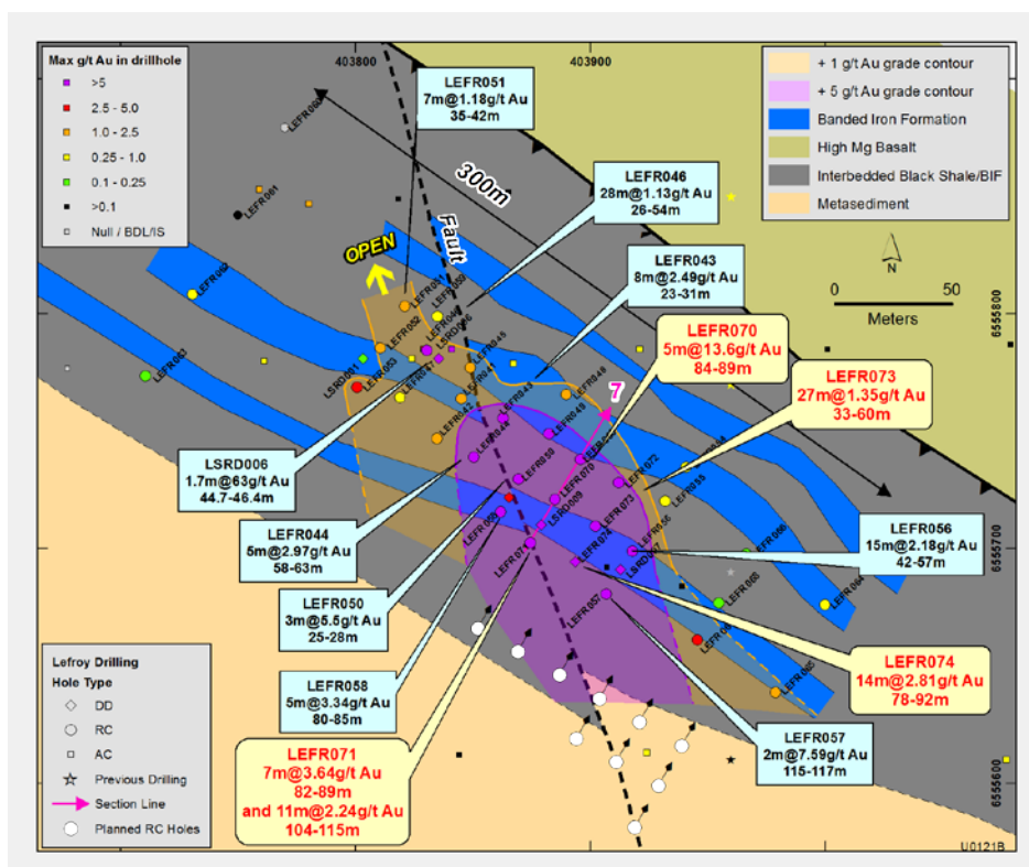
Figure 2 Lucky Strike geology and drill hole plan, highlighting previous drilling and planned step out RC drill program.
