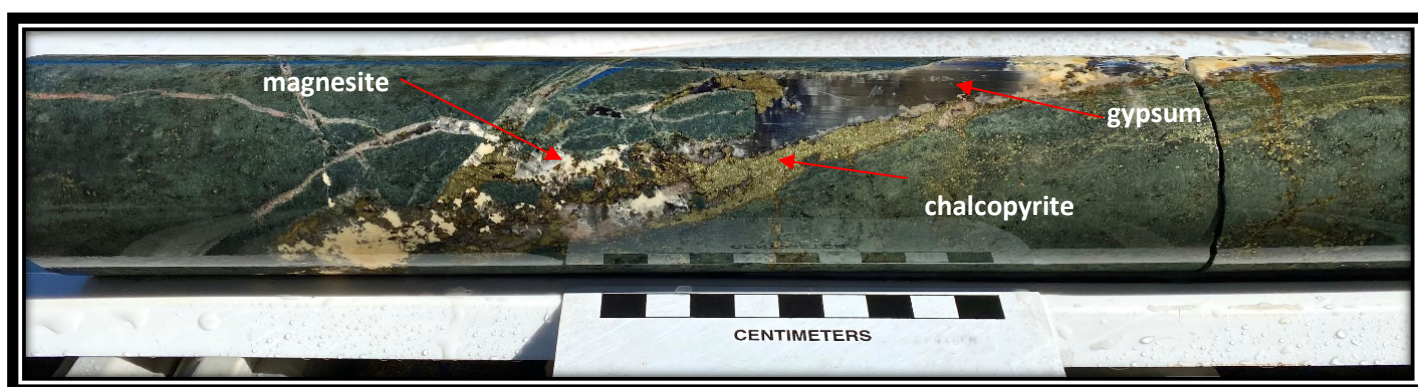
Figure 5 LEFRD267 interval 301 – 301.3m showing chalcopryrite in association with a gypsum magnesite vein in basalt.
