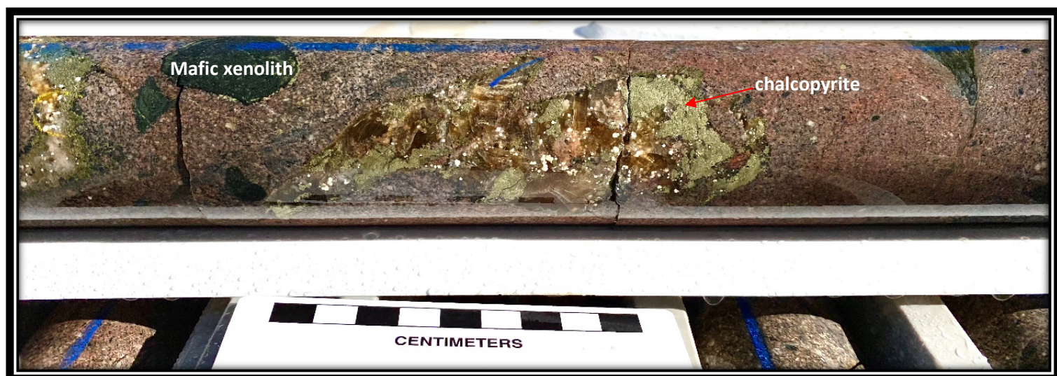
Figure 8 Close up LEFRD267 interval 311.3 – 311.4m showing chalcopryite with anhydrite, magnesite and strong hematite (red) alteration in quartz feldspar porphyry and the mafic xenolith
