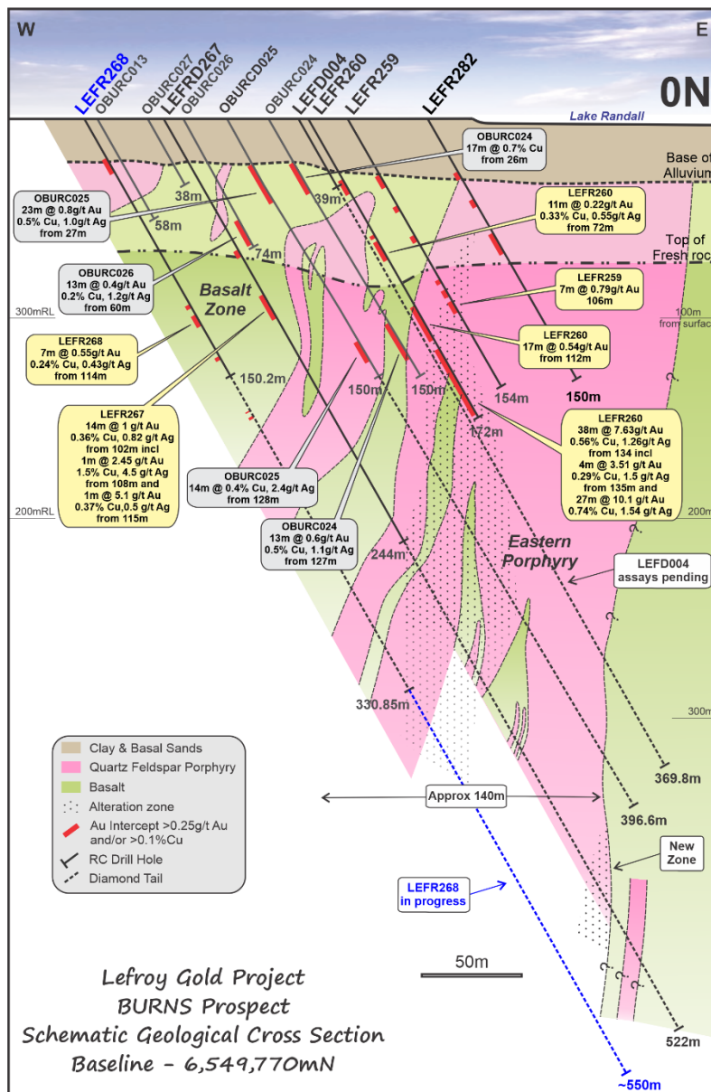
Figure 3 Baseline drill section ON highlighting position of hole LEFRD267 and the extension to hole LEFR268 (blue dash line) that is currently underway to evaluate the Eastern Porphyry
