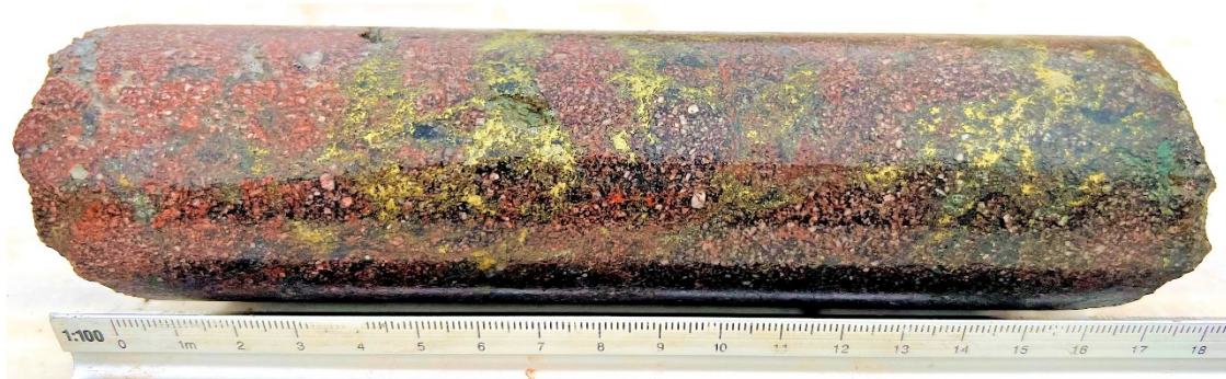
Figure 5 LEFD006 interval 435.6-435.8m showing Burns diorite porphyry altered by pervasive hematite, cross-cut by chalcopyrite and pyrite stringer veining (LEX ASX release 1 August 2022).
