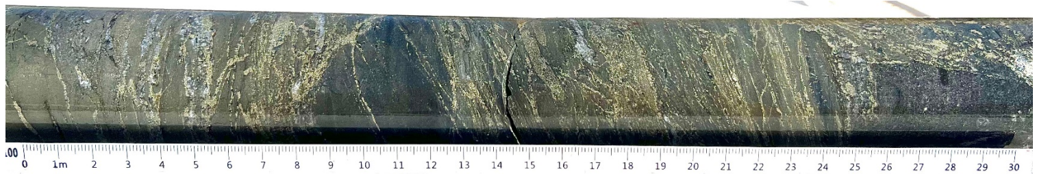
Figure 6 LEFD006 interval 1031.95-1032.25 4 Carbonate and quartz altered siltstone. Sub massive pyrite and pyrrhotite with rare chalcopyrite
