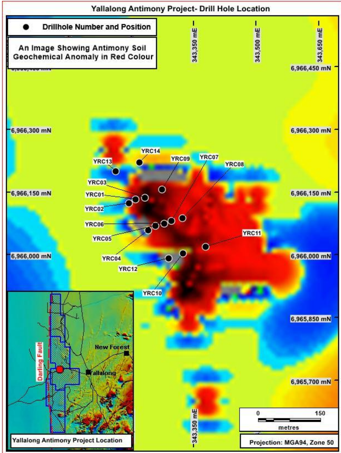
Figure 1. Yallalong Antimony Project showing drill hole locations over an antimony soil geochemical anomaly (shown as red colour).
