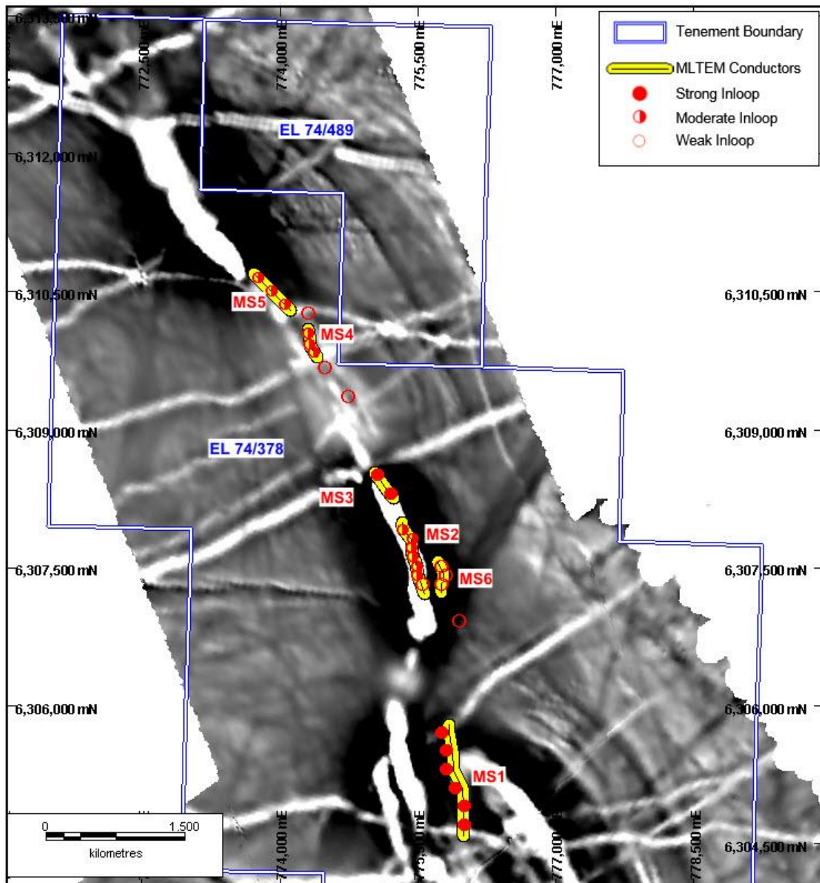
Figure 2. Greyscale aeromagnetic image showing the position of the MS1 to MS5 electromagnetic targets.
