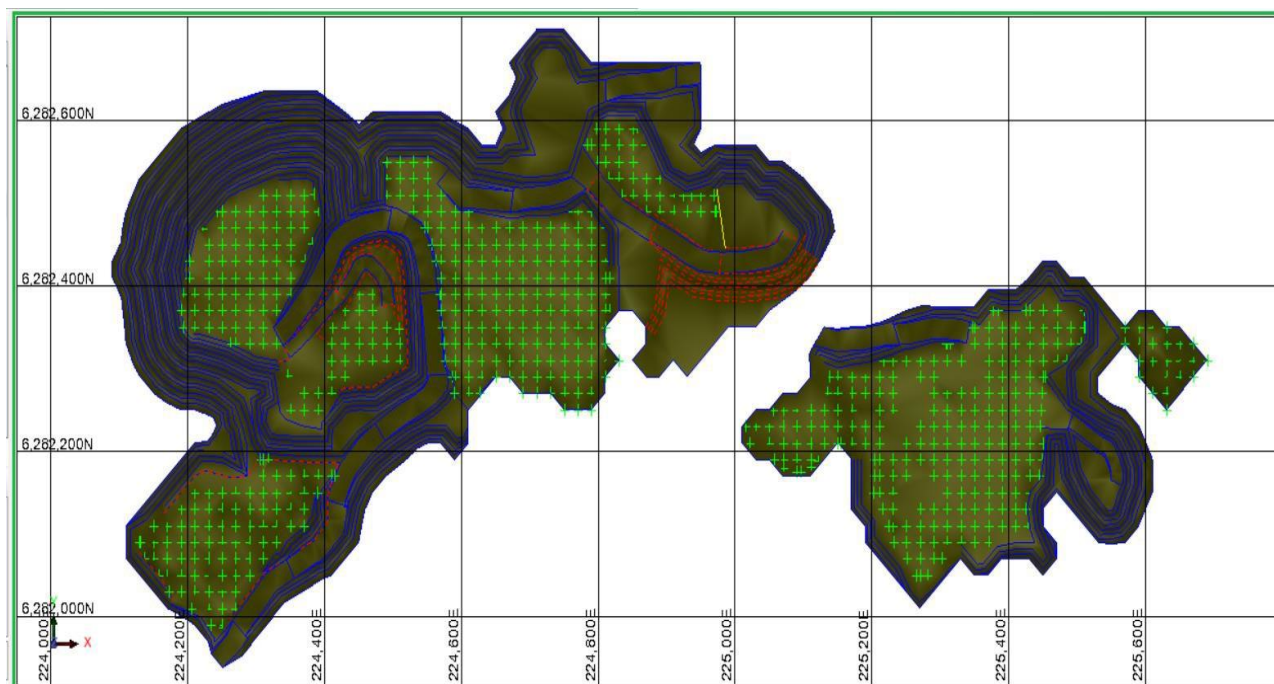
Figure 3: Current optimized pit design.
