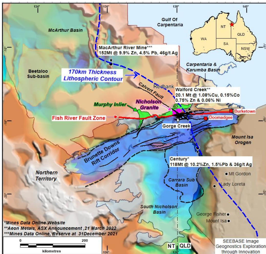
Figure 1: A SEEBASE image showing the position of the Gorge Creek Project in relation to the Murphy Inlier, South Nicholson Basin, MacArthur Basin and the Brunette Downs Rift Corridor
