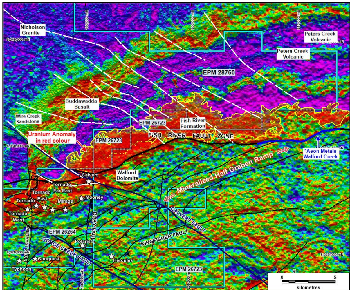
Figure 2. A U 2 /Th ratio radiometric image over Gorge Creek highlighting in red the main uranium anomaly coincident with the Fish River Formation (yellow boundary) north of the Fish River Fault. Numerous other anomaly positions also show along fault lines
