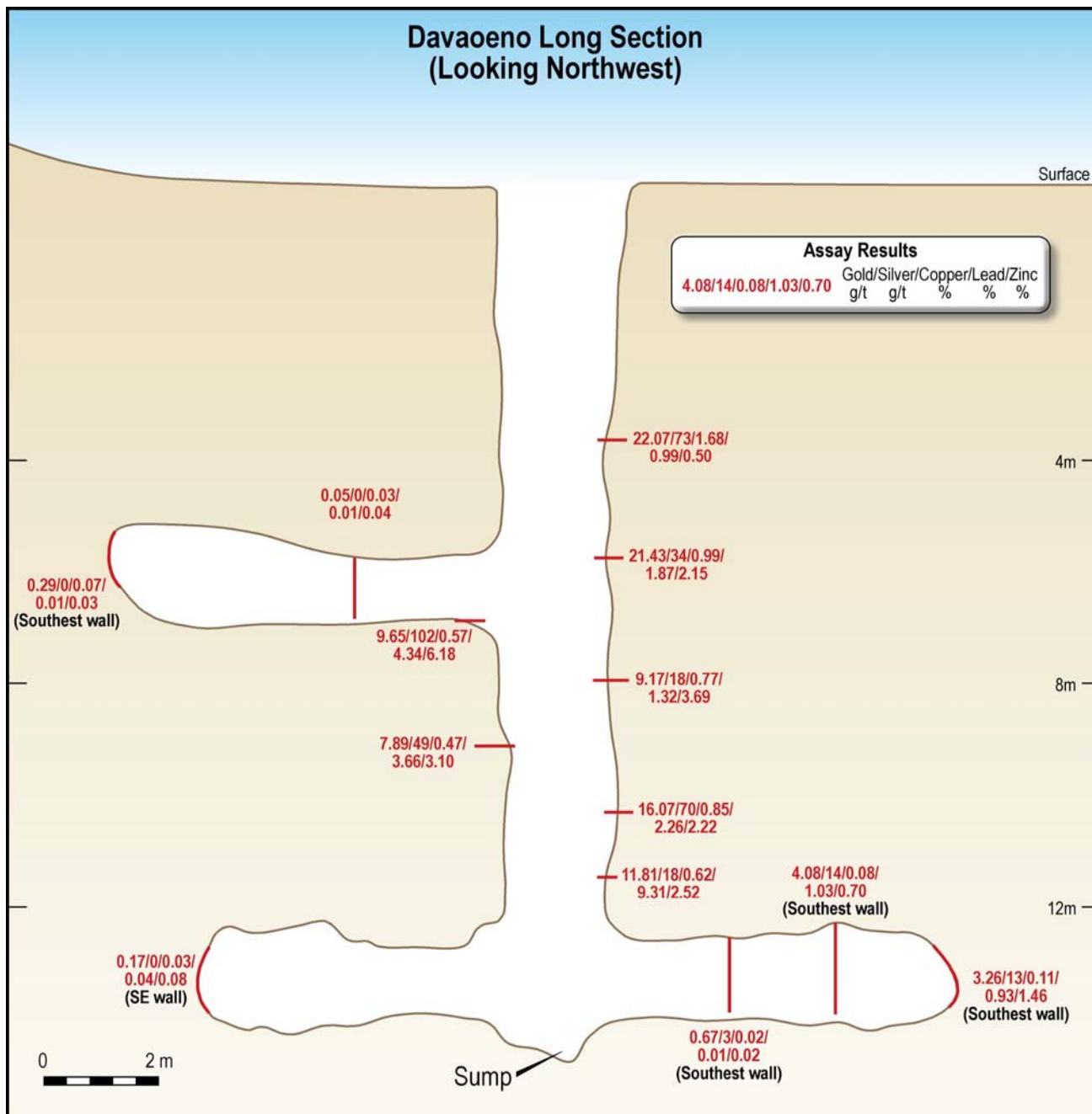
Figure 3: Davaoeno Mine – longitudinal section
