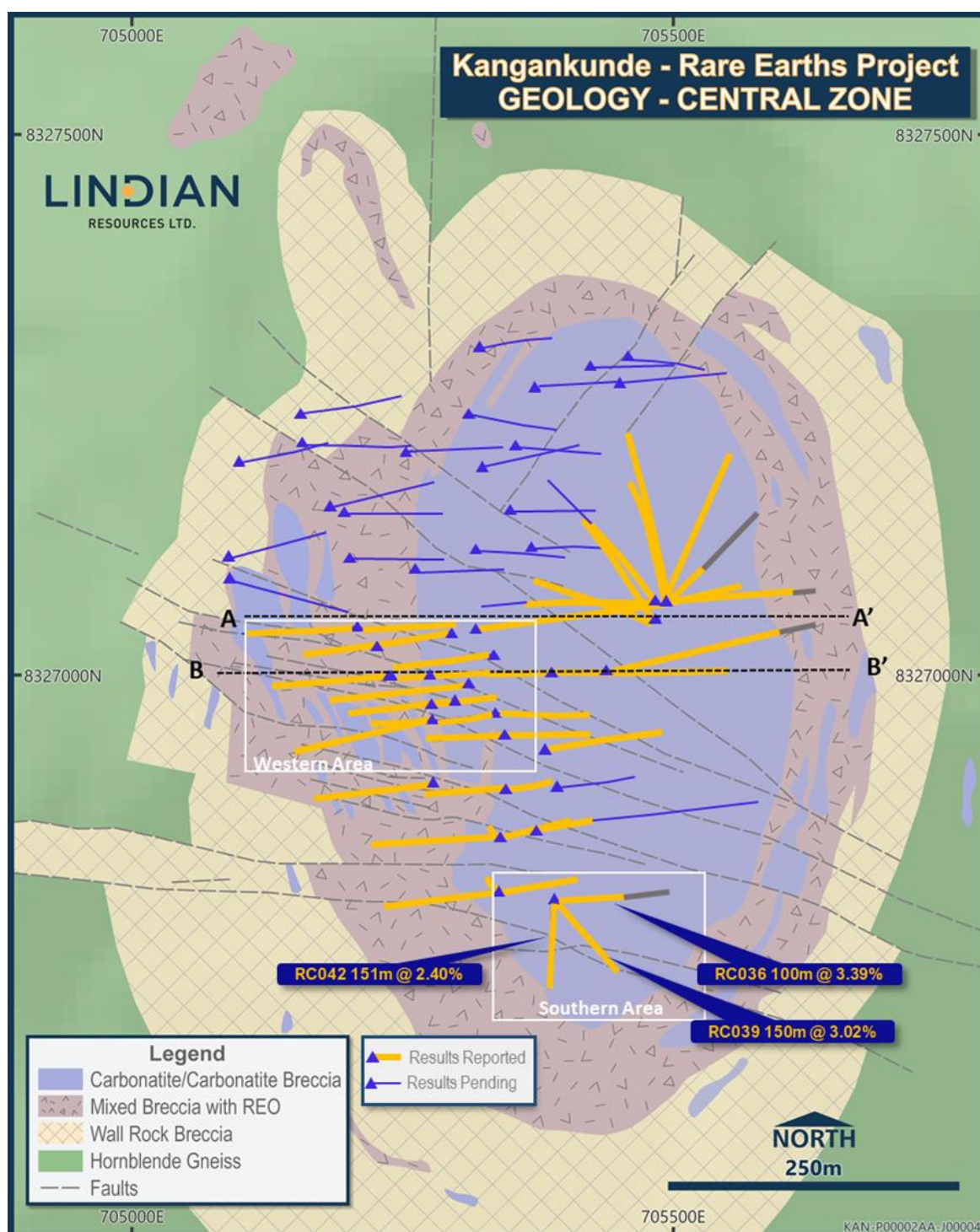
Figure 4: Kangankunde central carbonatite geology plan and drilling locations.
