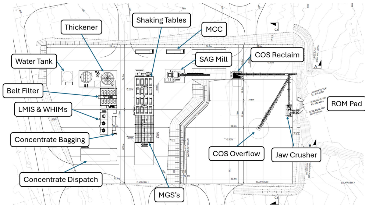
Figure 10: Process Plant highlighting the location of key packages
