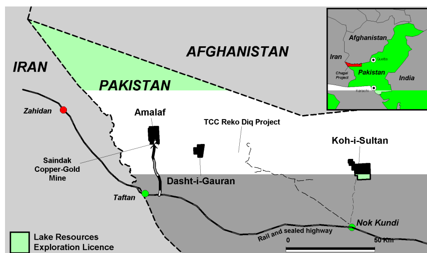
Figure 1: Location and tenement map.
