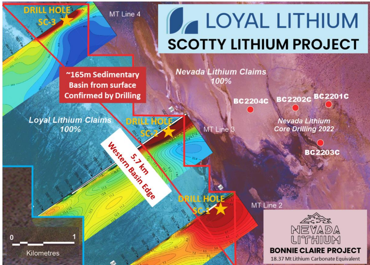
Figure 4: Scotty Lithium Target 2 Sedimentary Basin – MT traverses projected to the horizontal
