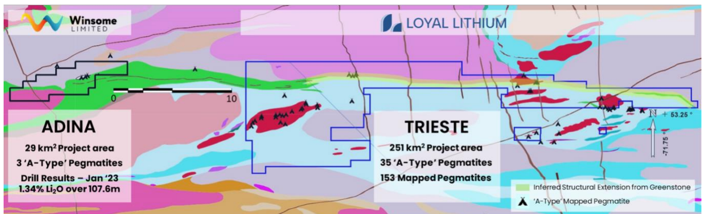
Figure 3 – Trieste Lithium Project – GSQ Region Interpretation (1:100k)
