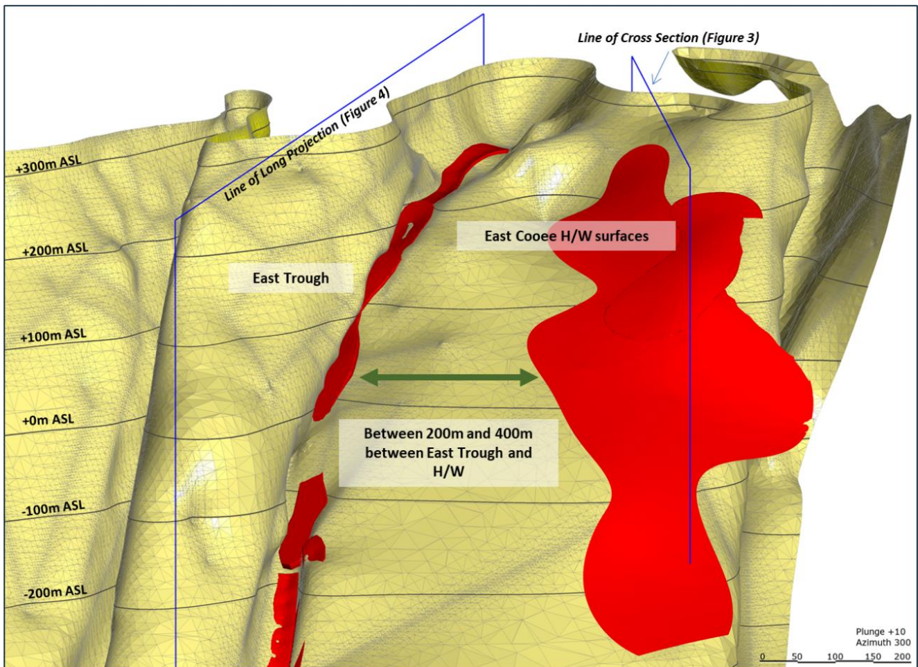
Figure 2: East Cooee area – perspective view looking (NW) illustrating spatial relationship between East Trough, East Cooee H/W (geological solids red) and the Lunnion Basalt contact (mesh -tan coloured)
