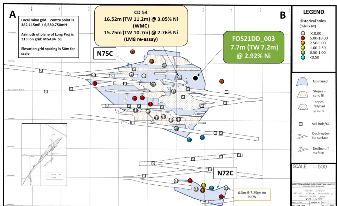
Figure 1: Representation of WMC Resources Longitudinal Projection for the N75C & N72C nickel surfaces at the Foster Mine, KNP (looking north east) 1 .
