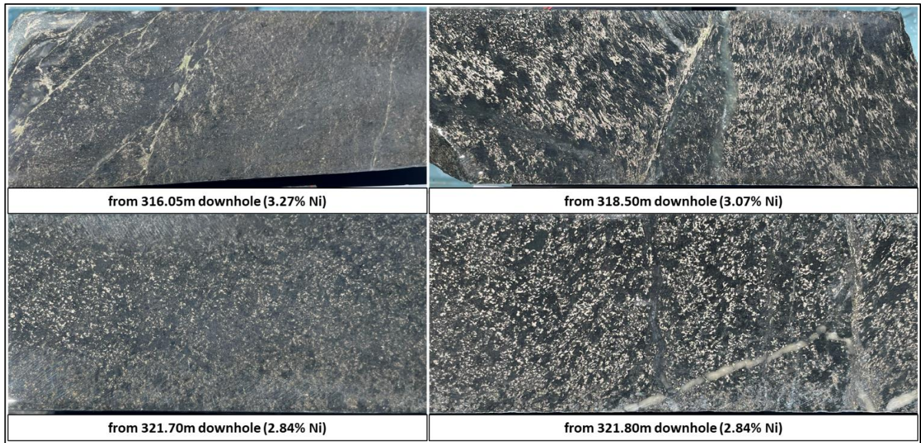
Figure 2: Photo-mosaic – grades of nickel sulphides in FOS21DD_003 – images show from downhole depth – for scale core/image width is 50mm
