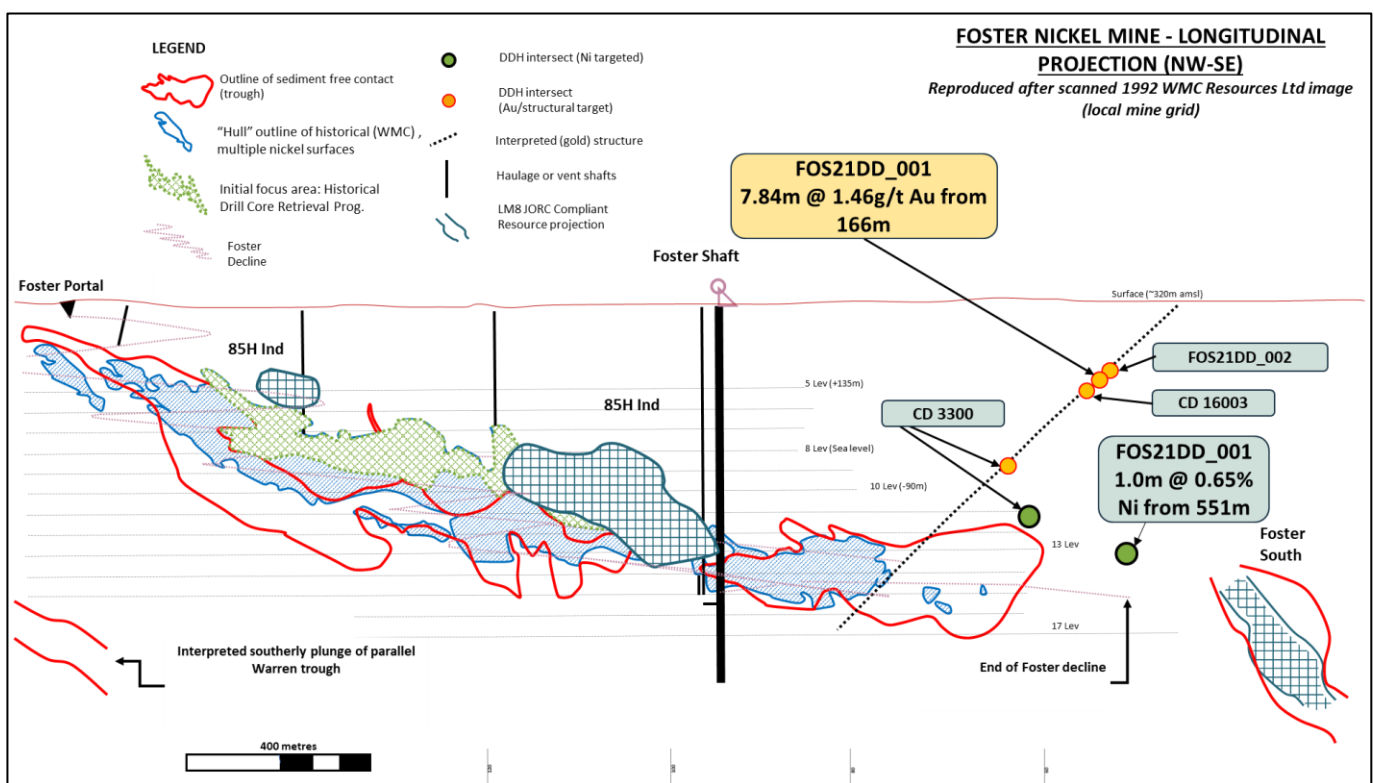
Figure 3: Longitudinal Projection of Foster Mine (looking north-east) illustrating the intersection points of reported Foster Gap diamond drill holes, related to both gold and the prospective nickel contact.
