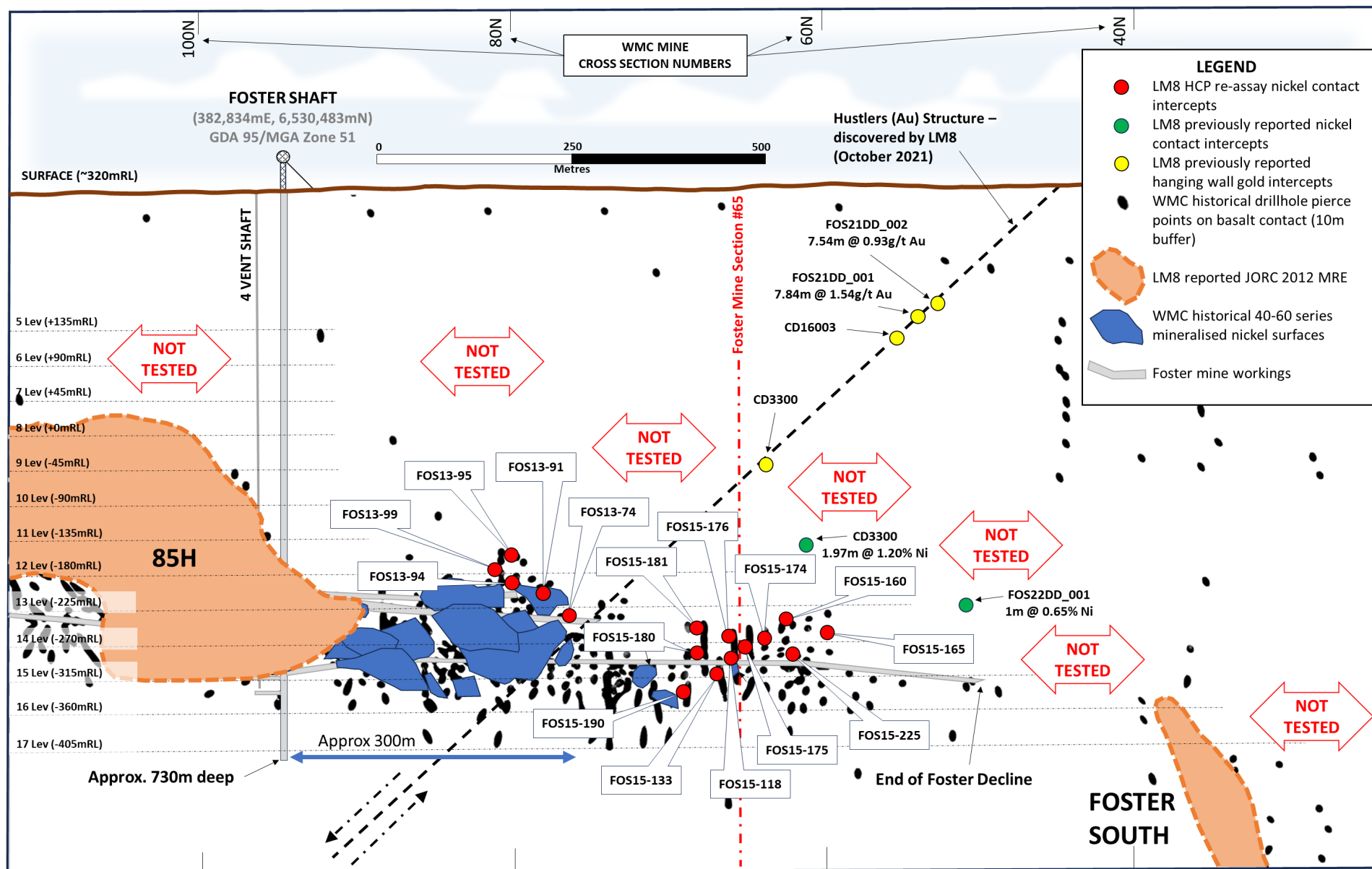
Figure 1: Long projection view of the southern end of the Foster nickel mine illustrating location of reported assay results, Lunnon Metals' 85H and Foster South nickel MRE areas adjacent to historical WMC mineralised areas (blue), Foster Shaft and decline and previous Company surface DD completed in 2021/2022 (view looking towards 045° north-west to left of image).
