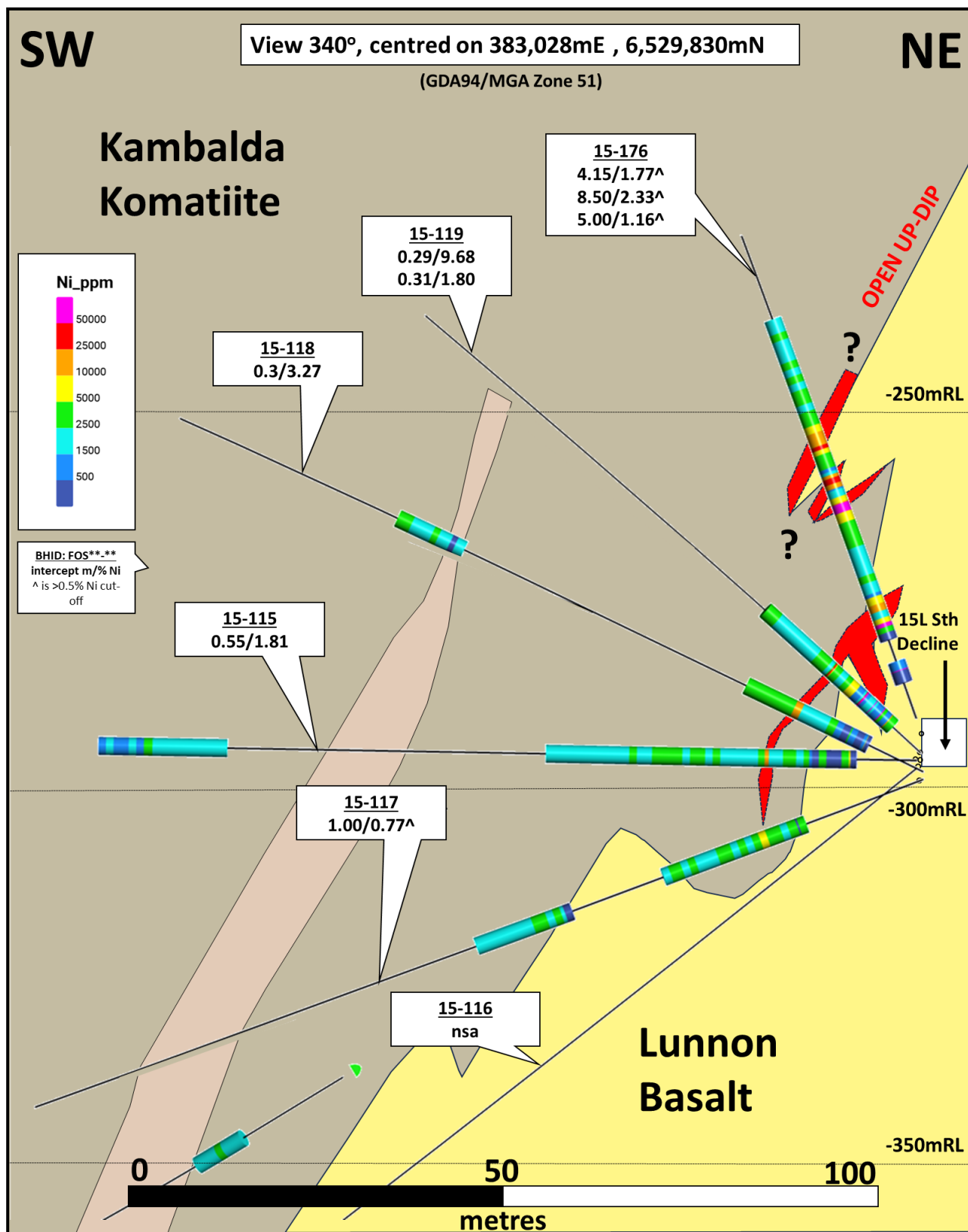
Figure 2: Cross-sectional view of Foster Mine Section #65 illustrating historical and current re-assay results for past WMC underground drilling.
