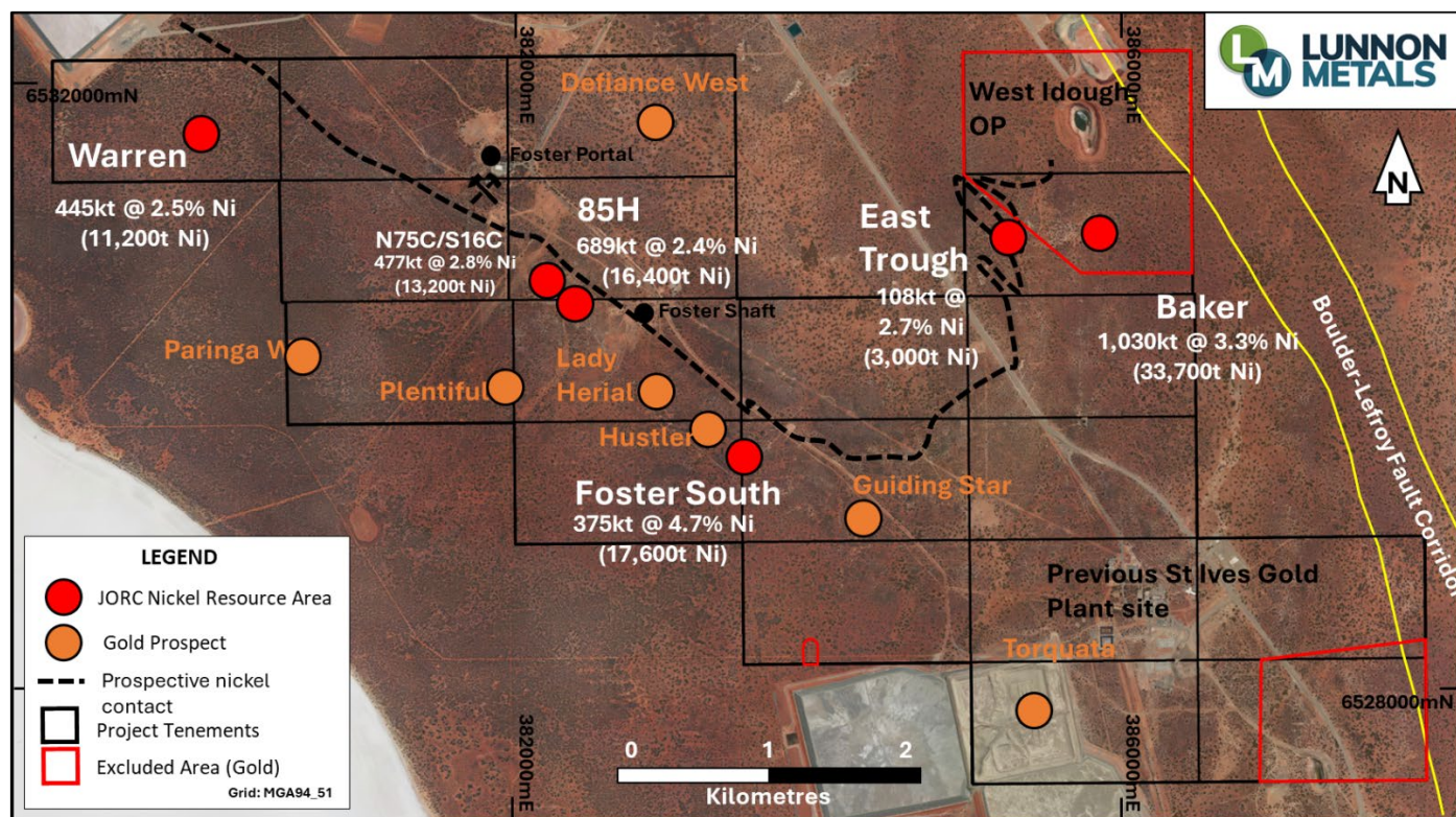
Figure 3: Foster-Baker Project Area showing nickel Mineral Resource 11 positions and select gold prospects.
