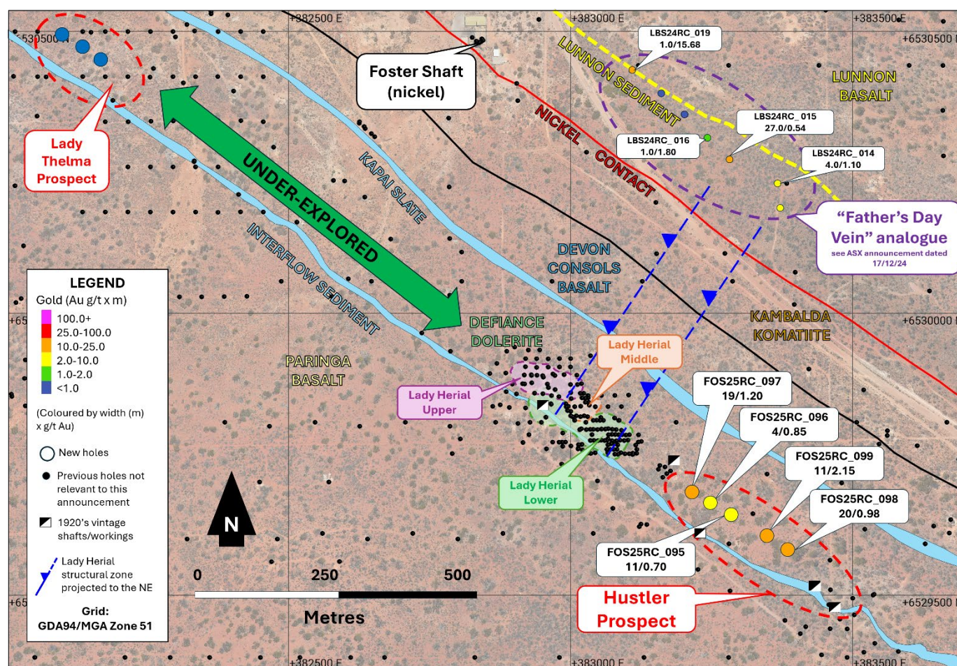
Figure 1: Plan view at the Lady Thelma to Hustler portion of the Foster Gold Belt, showing Lady Herial and two areas drilled in latest RC program.
