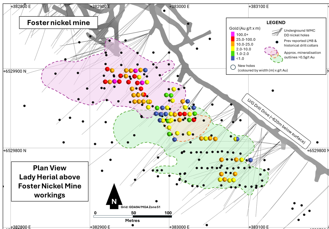
Figure 2: Plan view of the Lady Herial gold mineralisation outlines and the assay results reported today (coloured spheres) illustrating the location of the Foster nickel mine workings, some 620m below.
