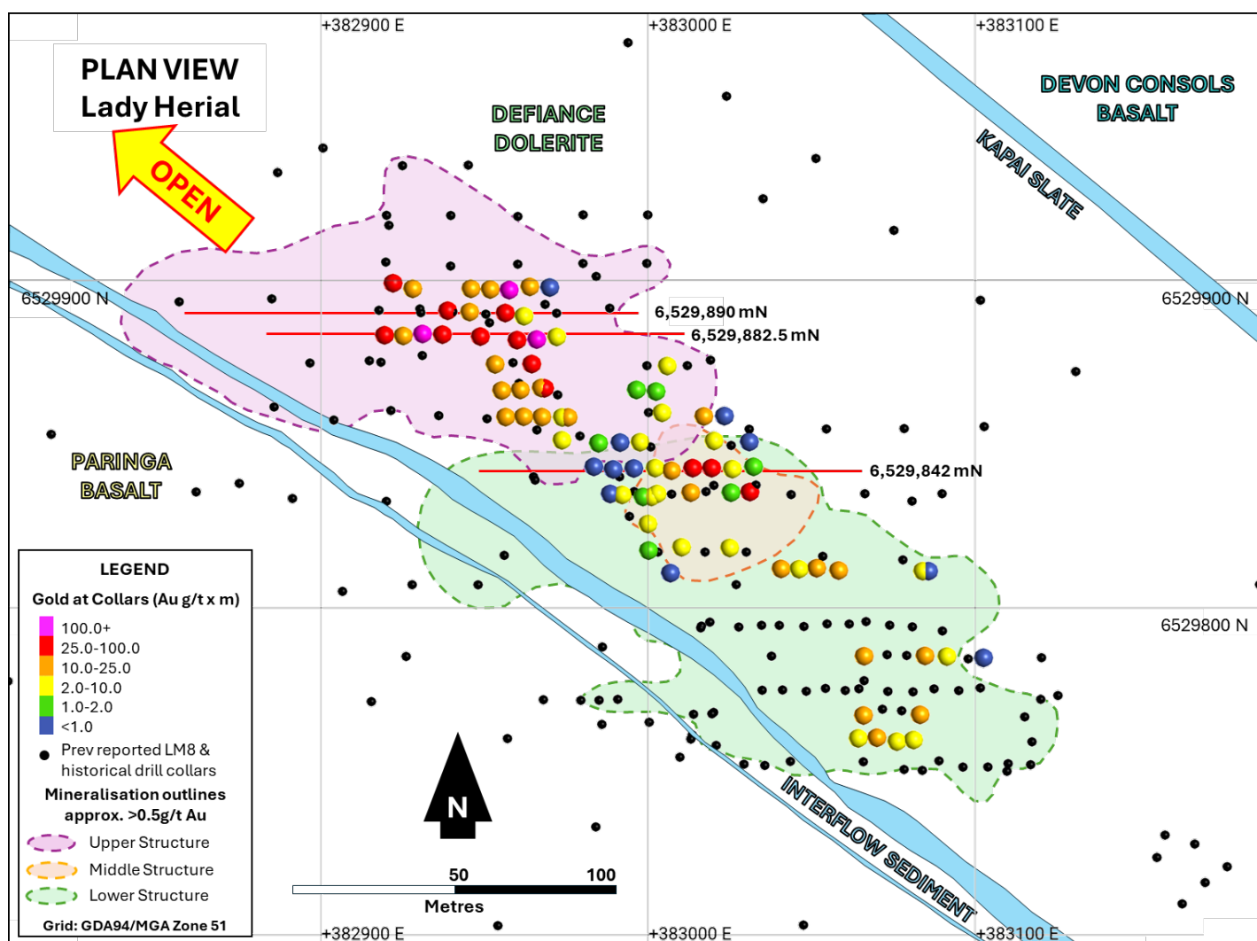
Figure 1: Plan view at the Lady Herial deposit scale, illustrating today's results (coloured spheres) drilled in latest RC campaign.
