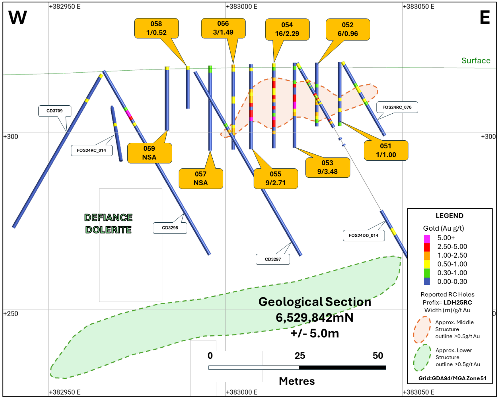
Figure 5: Geological cross section 6,529,842mN
