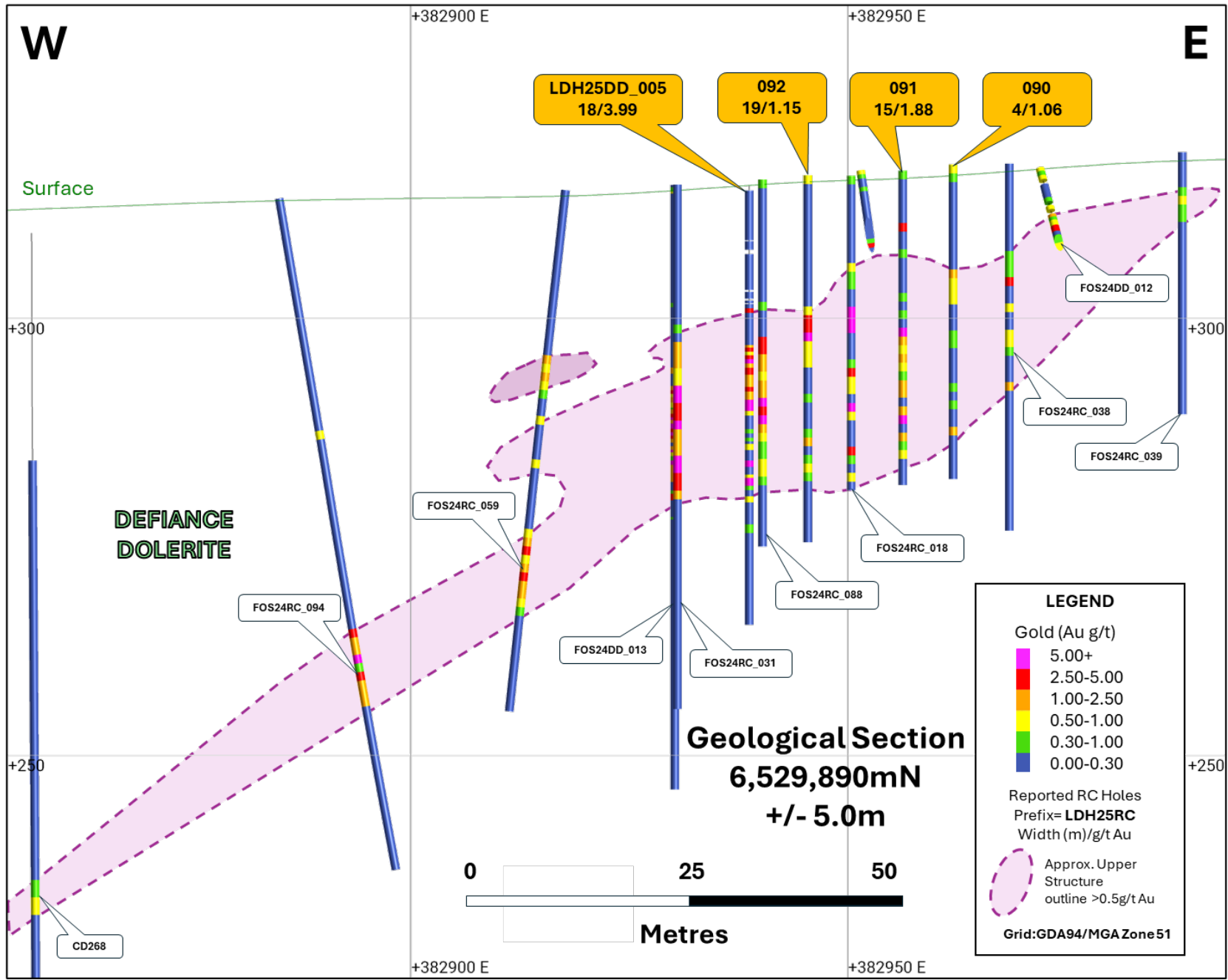
Figure 4: Geological cross section 6,529,890mN
