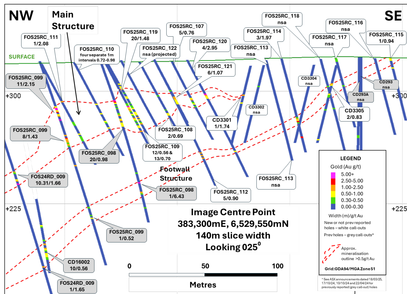
Figure 1: Long projection (looking northeast +/- 70m) illustrating the significant Hustler results reported today (white call-outs) and prior reported results (grey call-outs).
