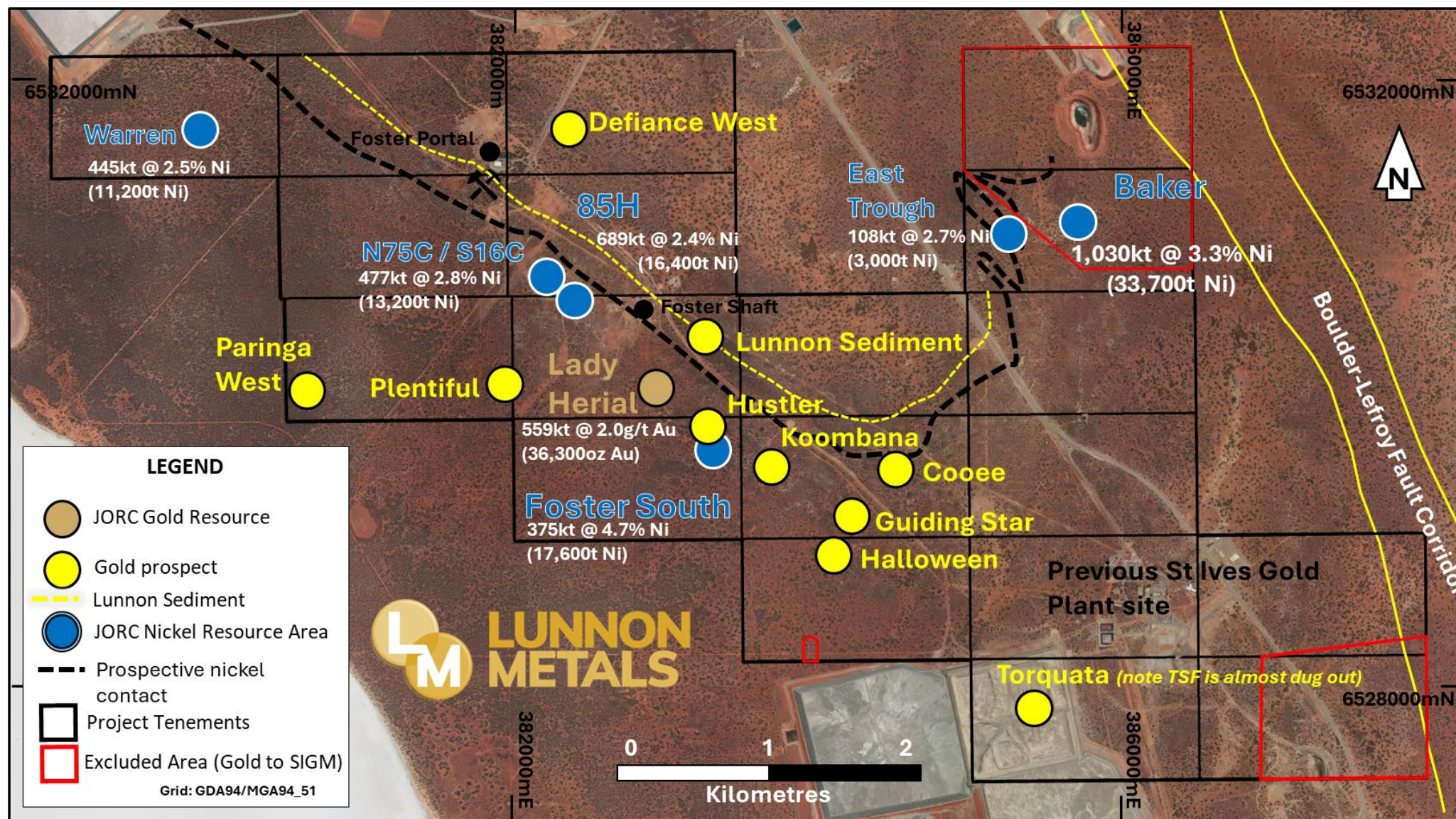
Figure 4: Foster-Baker Project Area showing location of Paranga West and select high-ranking gold prospects, gold & nickel Mineral Resource 5 positions.
